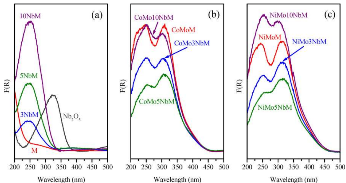
Fig. 5. UV-vis DR spectra of the x NbM supports (a), \text{CoMoxNbM} (b) and \text{NiMoxNbM} (c) catalysts, where x represents Nb loading in the supports (0, 3, 5 and 10 wt.%). The spectrum of the bulk \text{Nb}_2\text{O}_5 obtained after the calcination of ammonium niobate(V) oxalate hydrate at 500^\circ\text{C} for 4 h is also included in (a).
