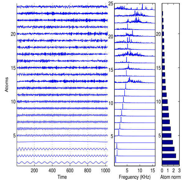
Fig. 8. A selection of learnt atoms in time (left) and frequency (middle) domain. Their norms are shown in the right panel.
