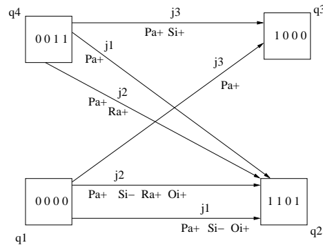
Figure 1. State transition diagram for the scenario
