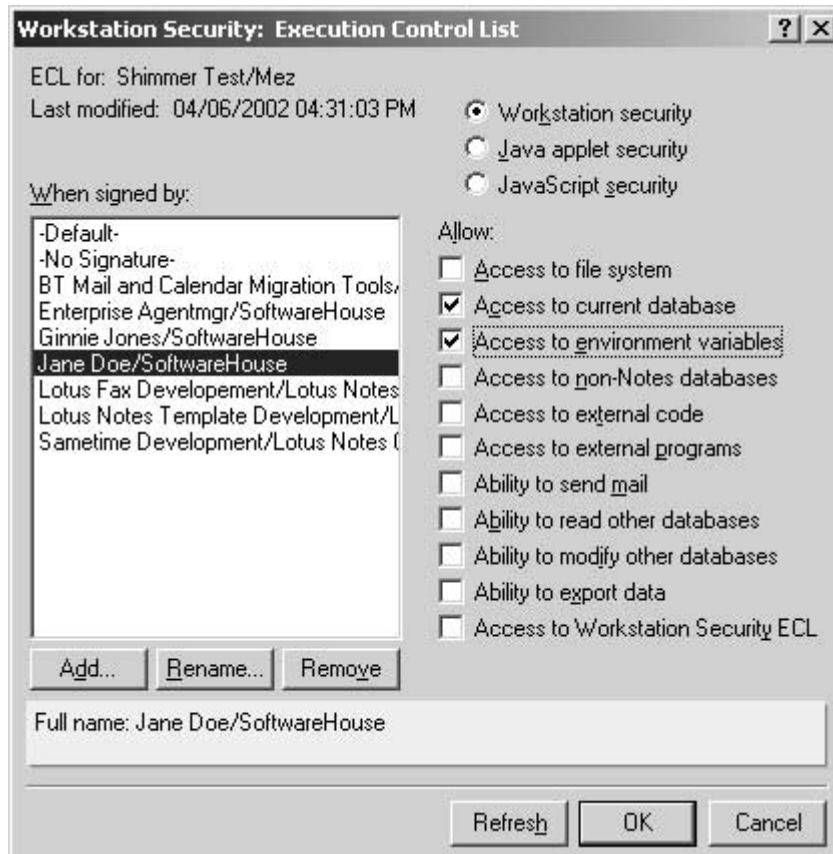
Figure 1: Lotus Notes Execution Control List
