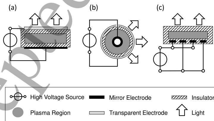
Figure 5. DBD modules for the generation of light (cross sectional sketches): (a) sealed planar and (b) cylindrical excimer lamp configurations; (c) coplanar excimer lamp configuration ©(all subfigures) 2006 Elsevier. Reproduced with permission from [132]
