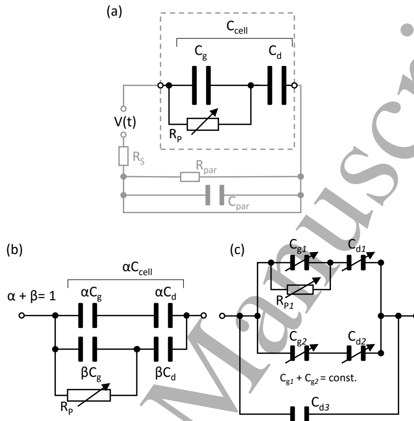
Figure 10. Advanced equivalent circuits for DBDs: (a) circuit including stray or parasitic elements; (b) partial discharged volume DBD ©2015 IOP Publishing. Reprinted, with permission, from [48]; (c) surface DBD actuator [288]; (b) and (c) can also be affected by external elements (see outside the dashed box in part (a))
