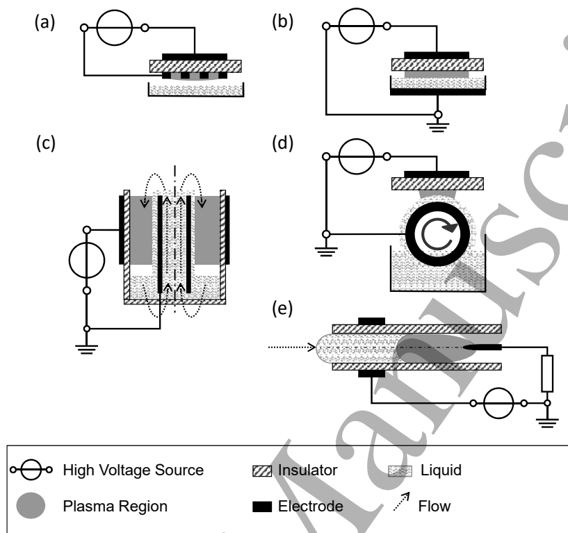
Figure 8. Schemes for DBD-based treatment of liquids: (a) indirect treatment by means of surface barrier discharge [169]; (b) direct treatment, i.e. liquid serving as one electrode [174]; (c) water falling film reactor [175]; (d) rotating drum reactor [179]; (e) liquid electrode DBD [181]
