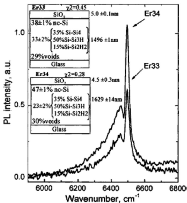
FIG. 5. PL spectra of nc-Si:H (%H=27%–28%) with different nc-Si densities and doped with Er (%Er=0.1%).
