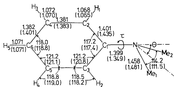
FIG. 1. Geometrical parameters and optimized geometries of DMA and DMA + . Bond distances are in \text{Å} and angles in degrees.
