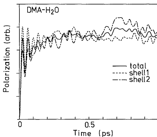
FIG. 7. Nonequilibrium simulation results for the DMA–H 2 O solution. (a) Solvent shell components of the solvation coordinate s(t) . (b) s(t) divided into the inter- and intramolecular terms. (c) Solvent shell components of the polarization P_r(t) . In (a), (b), and (c), solid lines are total s(t) or P_r(t) . Dashed and dashed–dotted lines correspond to first and second shell components in (a) and (c), and to V_1^{\text{int}} - V_0^{\text{int}} and V_1^{\text{DMA}} - V_0^{\text{DMA}} in (b).
