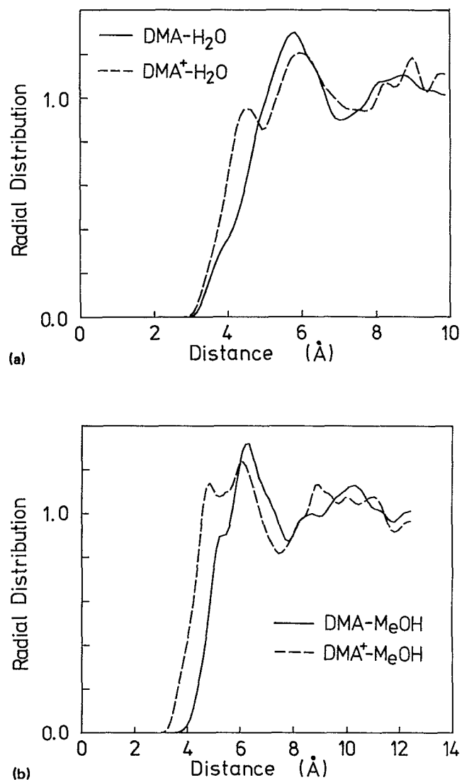
FIG. 4. Radial distribution functions between centers of mass of DMA (DMA + ) and (a) H 2 O and (b) MeOH. Solid and dashed lines correspond to DMA and DMA + , respectively.
