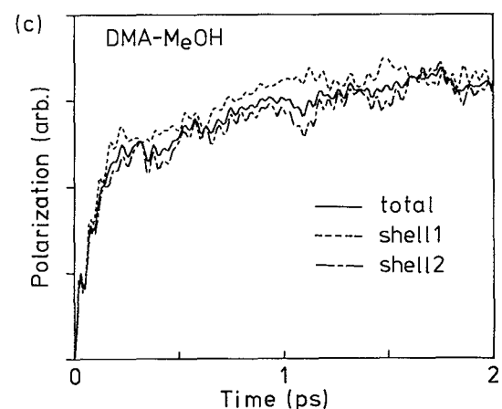
FIG. 8. Nonequilibrium simulation results for the DMA-MeOH solution. (a), (b), and (c) are similar to Fig. 7.
