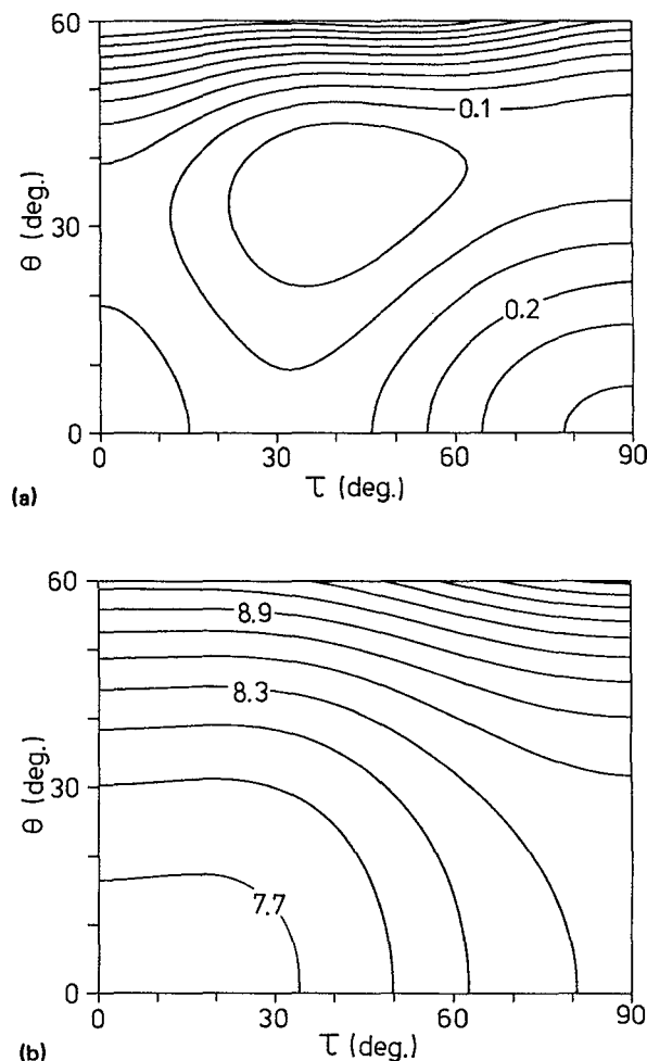
FIG. 2. Contour maps of potential energy surfaces of (a) DMA and (b) DMA + . Energy at the minimum of the DMA + potential surface is 7.6 \text{ eV} . Contour spacings are 0.05 and 0.2 \text{ eV} for DMA and DMA + potential surfaces, respectively.
