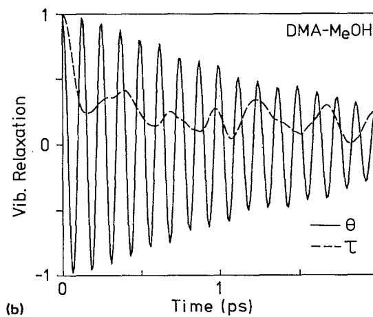
FIG. 9. Vibrational relaxation of \theta and \tau in (a) water and (b) methanol solutions. Solid and dashed lines correspond to \theta and \tau , respectively.
