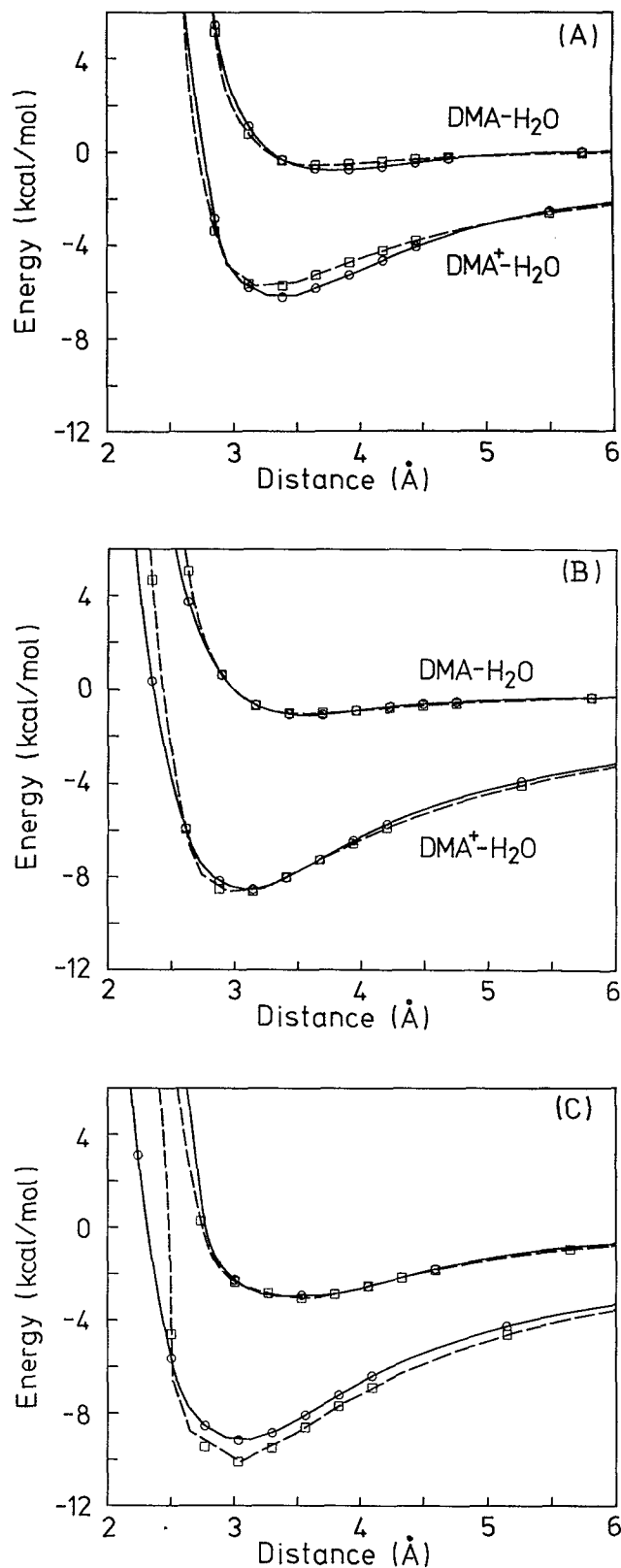
FIG. 3. DMA(DMA + )-H 2 O intermolecular potential energy curves. Symbols \circ (solid lines) are computed values from MO calculations and \square (dashed lines) by Eq. (2.2) with optimized potential parameters. The abscissas denote the distance from the O atom in H 2 O to (A) the midpoint of two methyl C atoms; (B) the C 6 atom in the phenyl ring; and (C) the NC 1 line of the DMA molecule, respectively. For the types of configurations (A), (B), and (C), see the text.
