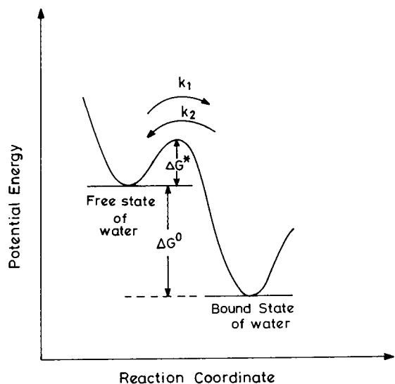
Figure 2. Schematic potential energy diagram showing the free water state, bound water state, and activated complex for the dynamic equilibrium [\text{H}_2\text{O}]_{\text{free state}} \rightleftharpoons [\text{H}_2\text{O}]_{\text{bound state}} versus the reaction coordinate. The \Delta G^0 is the difference in the free energy of a hydrogen bond of a water molecule between a biomolecule and a solvent water. 32 The \Delta G^* is the energy of activation.
