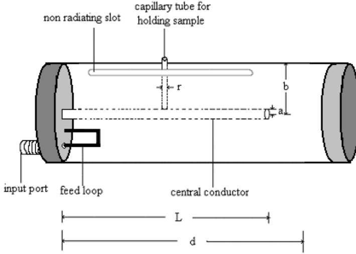
Figure 1. Schematic diagram of the coaxial cavity resonator.
