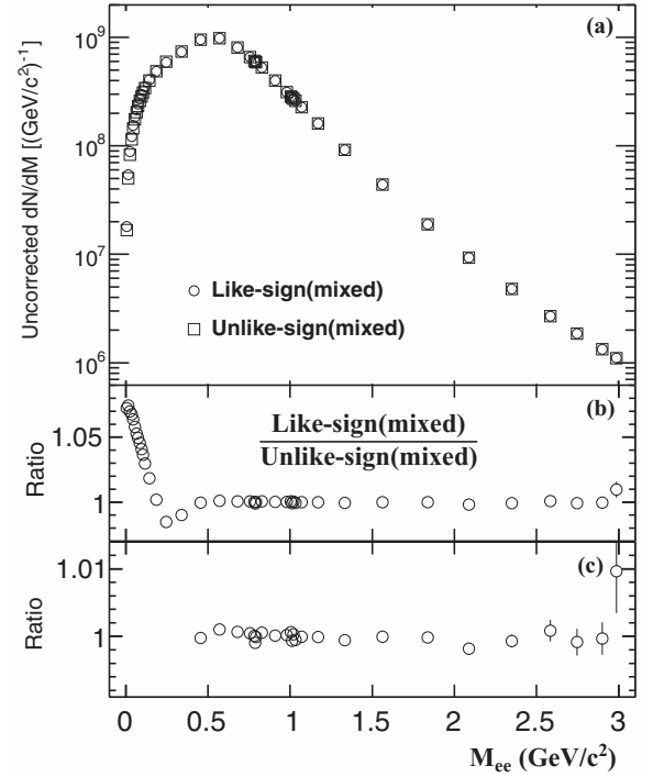
FIG. 3. (a) The mixed-event unlike-sign and mixed-event like-sign electron pair invariant mass distributions in minimum-bias Au + Au collisions at \sqrt{s_{NN}} = 200 GeV. (b) The ratio of mixed-event like-sign distribution to mixed-event unlike-sign distribution in minimum-bias Au + Au collisions at \sqrt{s_{NN}} = 200 GeV. (c) A zoom-in version of panel (b).
