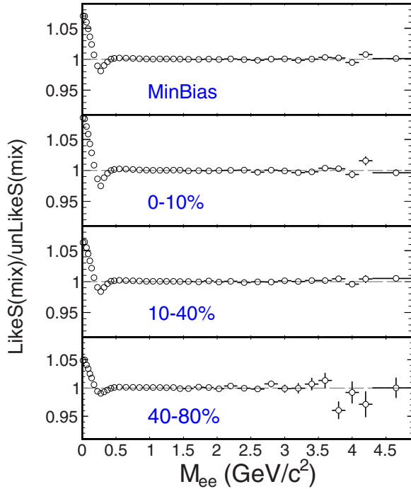
FIG. 4. (Color online) The ratio of the mixed-event like-sign distribution to the mixed-event unlike-sign distribution in minimum-bias Au + Au collisions at \sqrt{s_{NN}} = 200 GeV, as well as specific centrality selections of the collisions.
