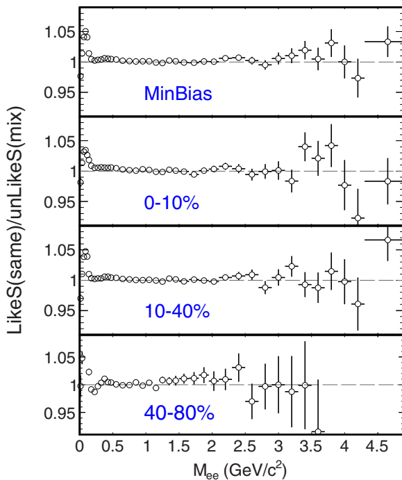
FIG. 7. (Color online) The centrality dependence of the ratio of the same-event like-sign distribution (corrected for the acceptance difference) to the normalized mixed-event unlike-sign distribution in minimum-bias Au + Au collisions at \sqrt{s_{NN}} = 200 GeV.
