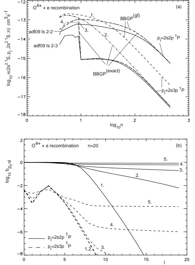
Fig. 2. \text{O}^{4+} recombination. a) Partial n -shell recombination coefficients: initial recombining metastable 2s^2 \ ^1S , intermediate excited parent p_i , final states (2s^2 \ ^1S)n with p_i = 2s2p \ ^1P and 2s3p \ ^1P . T_e = 1.6 \times 10^6 K, N_e = N_p = 0 . BBGP (gf) indicates use of standard cor_l matching the GF, BBGP (exact) indicates use of specific cor_l . For the \Delta n = 0 case, BBGP (gf) and BBGP (exact) are superposed. \Delta n = 1 cases: 1. no alternative Auger channels, GF cor_l ; 2. no alternative Auger channels, specific cor_l ; 3. 2s3p \ ^1P - 2s3s \ ^1S alternative Auger channel, specific cor_l ; 4. as before and 2s3p \ ^1P - 2s2p \ ^1P alternative Auger channel, specific cor_l . b) b_{p_i, n, l} factors for doubly-excited states of \text{O}^{3+} relative to \text{O}^{4+} 2s^2 \ ^1S for p_i = 2s2p \ ^1P and 2s3p \ ^1P , n = 20 , T_e = 10^6 K, N_e = N_p , plasma Z_{\text{eff}} = 1 . Cases: 1. N_e = 10^{10} \text{ cm}^{-3} ; 2. N_e = 10^{12} \text{ cm}^{-3} ; 3. N_e = 10^{13} \text{ cm}^{-3} ; 4. N_e = 10^{14} \text{ cm}^{-3} ; 5. N_e = 10^{15} \text{ cm}^{-3} . Note the alternative Auger channel reduction for the p_i = 2s3p \ ^1P graphs.
