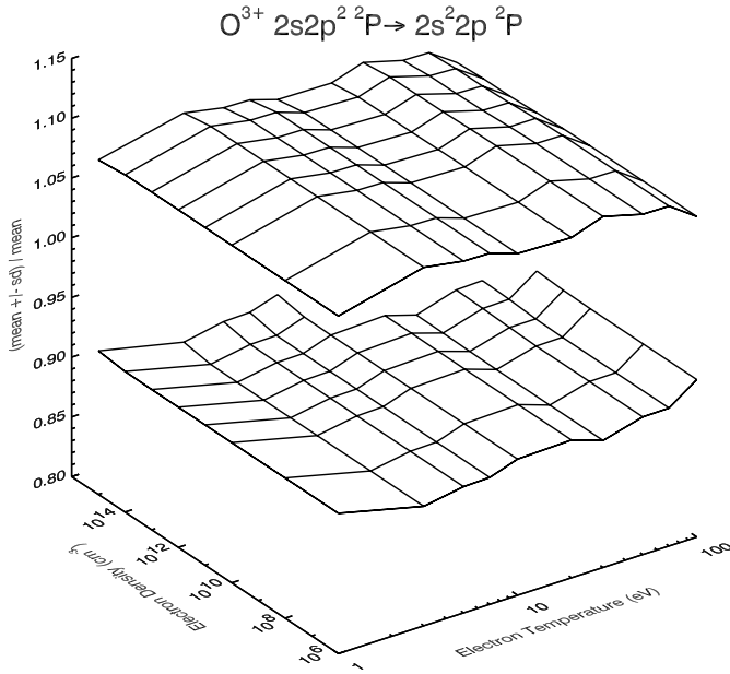
Fig. 7. Upper and lower cumulative statistical ( \pm 1 standard deviation) surfaces for the {}^{\text{R}}\mathcal{P}\mathcal{E}\mathcal{C}^z for the O IV 2s2p^2\ ^2\text{P} - 2s^22p\ ^2\text{P} multiplet at 554.4 Å. Note that projection has a substantial influence on the line emissivity and so its influence on the cumulative propagated error is significant. Projection and its error contribution is not included in the graph shown. \mathcal{P}\mathcal{E}\mathcal{C}^z data are archived in ADAS data format adf15 . The propagated “locked parameter” errors are available in .err files paralleling the .dat files for use in plasma modelling.
