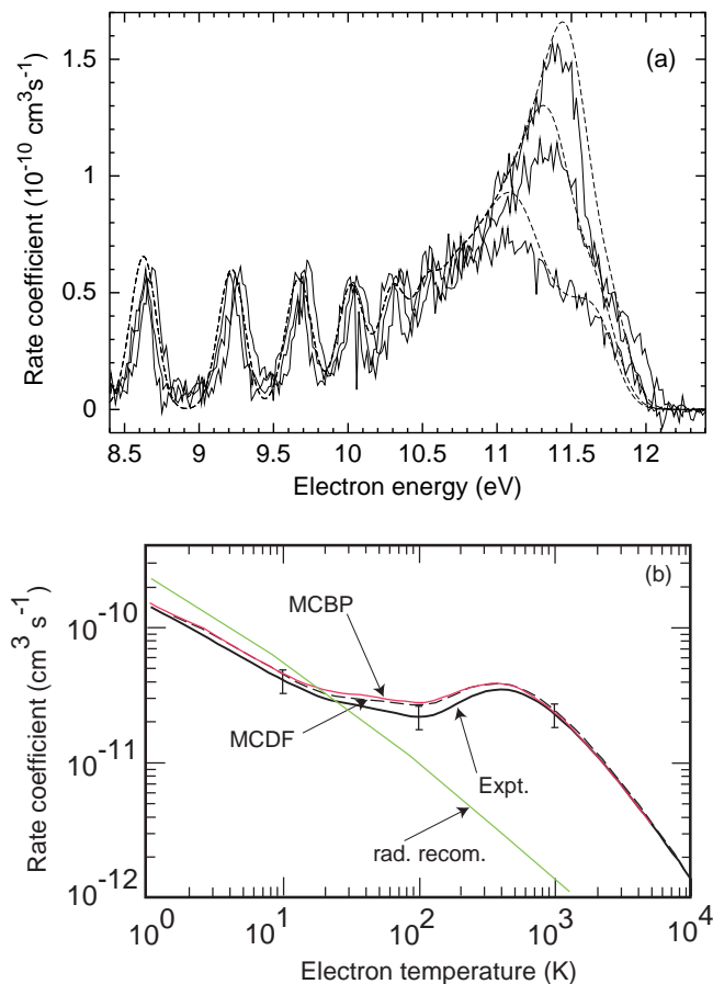
Fig. 3. a) A theoretical reconstruction is shown of the observed dielectronic recombination resonances for the light ion O^{5+} + e^- \rightarrow O^{4+} . The measurement is from the CRYRING heavy-ion storage ring (Böhm et al. 2002). Note that the dielectronic recombination data from the methods described in Sect. 2.2 have been convoluted with the experimental velocity distribution, which has the units of a rate coefficient. The three pairs of curves correspond to three different beam energies which results in three different cut-offs in the maximum principal quantum number detected. The experimental and theoretical data agree quite nicely. b) The Maxwellian dielectronic recombination rate coefficient for Fe^{18+} + e^- \rightarrow Fe^{17+} is shown. The measurement (solid curve) is from the Heidelberg storage ring (Savin et al. 2002a) with an experimental error assessed as \lesssim 20\% . The theoretical IPIRDW results include the 1 \rightarrow 2 , 2 \rightarrow 2 and 2 \rightarrow 3 core excitations in the multi-configuration Breit–Pauli (MCBP, dotted curve) and Dirac–Fock data (MCDF, dashed curve) with n_{\max} = \infty . The worst deviation from experiments is \lesssim 30\% (for the 3/3' resonances) with a typical uncertainty \lesssim 20\% for the direct state-selective coefficients to individual levels and for the total dielectronic rate coefficient. There is excellent agreement between the Breit–Pauli and Dirac–Fock results. The Breit–Pauli approach is used for our mass data production.
