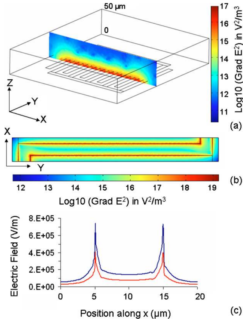
FIG. 1. (a) Contour plot of the gradient of the squared field, \nabla E^2 , generated across the gold IDE, up to 50 \mu\text{m} above the electrode's surface. (b) Contour plot of \nabla E^2 , simulated in the plane between two fingers separated by 10 \mu\text{m} . The DEP force is minimal in the middle of the gap and reaches a maximum value at the edge of the electrode's finger. The voltage between the electrodes is 2 V (peak). (c) Electric field cross section between two electrode fingers calculated for an applied voltage of 1.1 V (peak) (red) and 2 V (peak) (blue).
