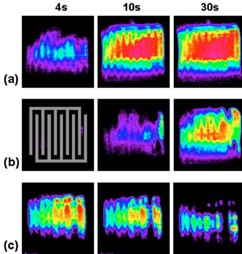
FIG. 5. Color coded TIRF images extracted from rRNA DEP movies at 4, 10, and 30 s after the onset of a 4 V_{p-p} ac field set at: (a) 100 kHz, (b) 3 MHz, and (c) 50 MHz measured after positive DEP at 100 kHz. Image processing included background subtraction and Gaussian smoothing. An outline of the electrode is superimposed on the first image of the 3 MHz series (enhanced online).
