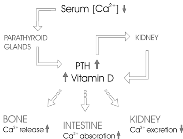
Fig 1. Regulation of calcium balance
