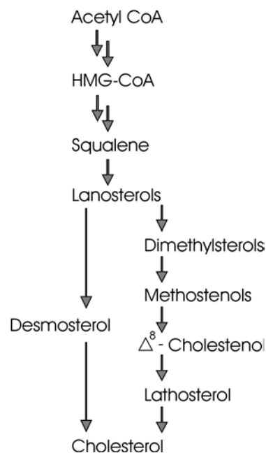
Fig 4. Synthesis of cholesterol (adapted from Relas 2000)
