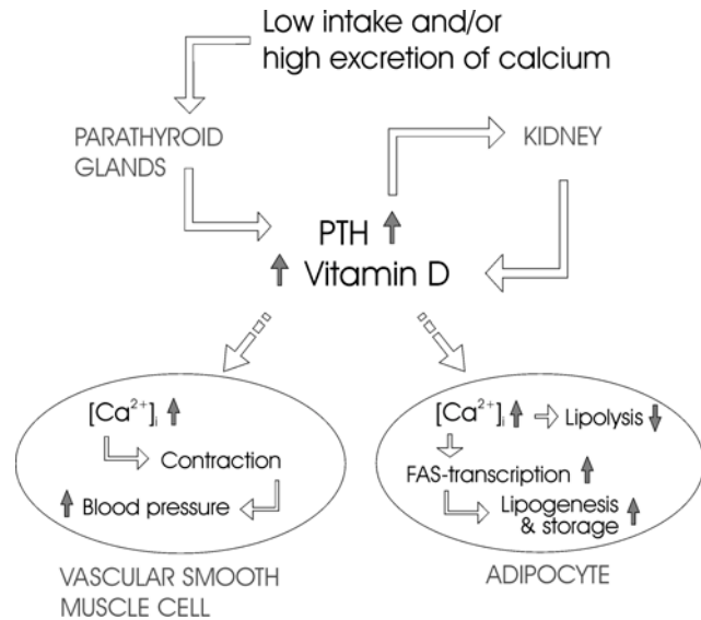
Fig 2. Suggested mechanism of the effects of dietary calcium on blood pressure and obesity (Zemel 2001)
