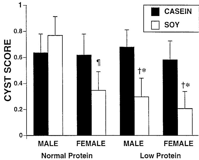
Figure 2. Effects of protein source, protein level, and gender on cyst score (% cyst area × right kidney weight/body weight) in pcy mice. There was a significant interaction between gender and protein source effects. † P < 0.05, protein source effect: significantly different from casein-fed animals of the same gender given the same level of protein. * P < 0.05 for males, P = 0.07 for females, protein level effect: significantly different from soy protein-fed animals of the same gender. ‡ P < 0.05, gender effect: significantly different from soy-fed males given the same level of protein.
