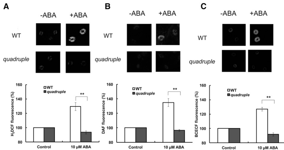
Figure 2. ABA-induced ROS and NO production and cytosolic alkalization in wild-type (WT) and pyr1/py11/py2/py4 quadruple mutant ( quadruple ) guard cells. A, ROS production. Representative grayscale H 2 DCF fluorescence images (top panel) and the percentage of H 2 DCF fluorescence levels (bottom panel) are shown. B, NO production. Representative grayscale diaminofluorescein (DAF) fluorescence images (top panel) and DAF fluorescence levels (bottom panel) are shown. C, Cytosolic alkalization. Representative BCECF images (top panel) and BCECF fluorescence levels (pH; bottom panel) are shown. Fluorescence intensities are normalized to the control value taken as 100% for each experiment. The epidermis was preloaded with fluorescent dyes before treatments. Ten micromolar ABA or 0.1% ethanol (solvent control) was added to the suspension of epidermal preparations for 20 min. Bars indicate averages of five independent experiments ( n = 5 ; a total of 100 guard cells per bar). Asterisks indicate significant differences (** \alpha = 0.01 ) by Student's t test. Error bars represent SE.
