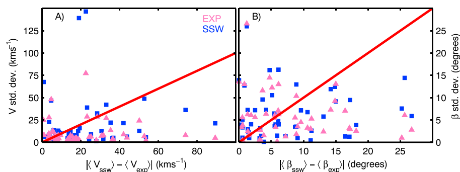
Figure 11. (a) Scatterplot comparing the standard deviation of the PPF, HMF, and SSEF speed estimates for the SSW (blue) and EXP (pink) profiles against the difference in the mean SSW- and EXP-derived CME speeds. The red line is the one-to-one line. (b) The same structure as Figure 11a but for CME direction estimates. In each case it is clear that more points lie below the one-to-one line than above, indicating that differences between the SSW and EXP profiles frequently cause larger differences in the speed and direction estimates than do the PPF, HMF, and SSEF techniques.
