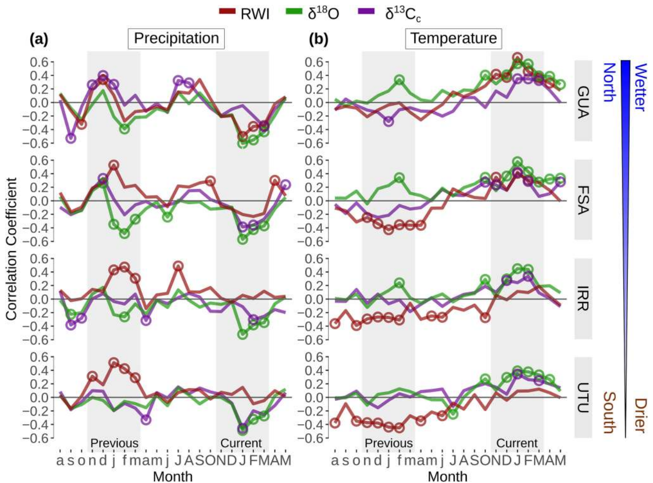
Figure 7. Summary of Pearson correlation coefficients between monthly regional (a) precipitation and (b) temperature and ring-width index (RWI), \delta^{18}\text{O} and \delta^{13}\text{C}_e tree-ring chronologies from August prior-year (lowercase) to May current-year (uppercase). Circles represent significant correlations and gray vertical shading highlight previous- and current-growing seasons.
