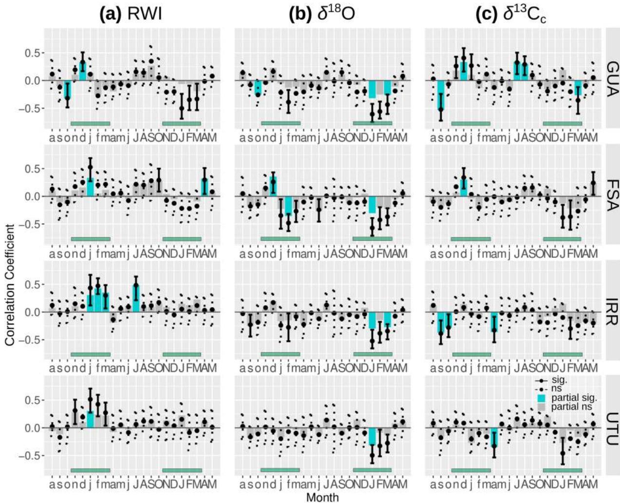
Figure 4. Correlation coefficients between monthly regional precipitation and (a) ring-width index (RWI), (b) \delta^{18}\text{O} and (c) \delta^{13}\text{C}_c tree-ring chronologies from August prior-year (lowercase) to May current-year (uppercase). Vertical lines represent bootstrap monthly correlations with solid lines indicating significant (sig.) and dashed lines nonsignificant correlations (ns). Bars represent partial monthly correlations where the relationship of each tree-ring variable (RWI, \delta^{18}\text{O} , \delta^{13}\text{C}_c ) and precipitation was computed after removing the covariability between precipitation and temperature. Colored bars indicate significant coefficients (partial sig.) and gray bars nonsignificant partial correlations (partial ns). Duration of the growing season is indicated by a green horizontal line.
