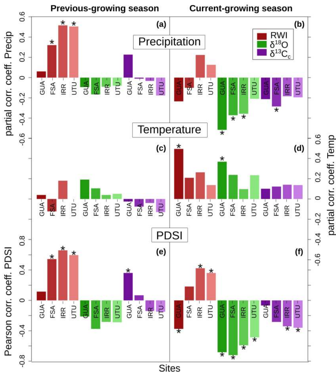
Figure 6. Correlation coefficients between the tree-ring width index (RWI), \delta^{18}\text{O} and \delta^{13}\text{C} chronologies and previous and current growing-season climate from November to March at the four study sites. For (a, b) precipitation and (c, d) temperature bars represent partial correlations that remove covariance between both climate variables, while correlations with (e, f) palmer drought severity index (PDSI) are simple Pearson correlations. Statistically significant correlations are indicated with stars (alpha = 0.05).
