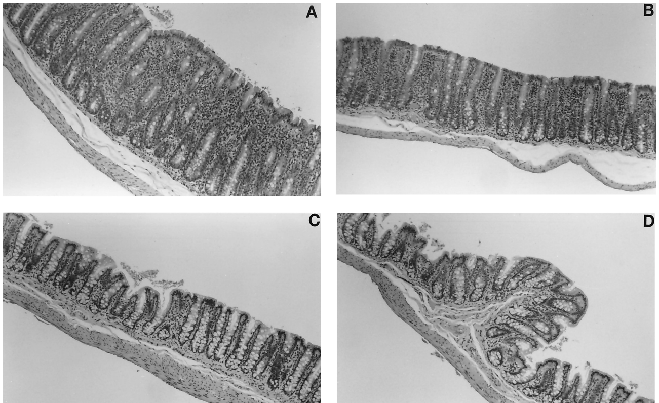
FIG. 2. (A) Photomicrograph of cecal inflammation in a 4-month-old SPF B27/ \beta_2 -microglobulin TG rat treated with water alone. (B) A TG rat treated with metronidazole after the onset of colitis (3 months of age) showed only slight reduction of cecal inflammation. (C) The cecum of a TG rat treated with vancomycin-imipenem after the onset of colitis (3 months of age) revealed substantially less cecal inflammation. (D) Normal cecum of a 4-month-old NT control rat treated with water alone.
