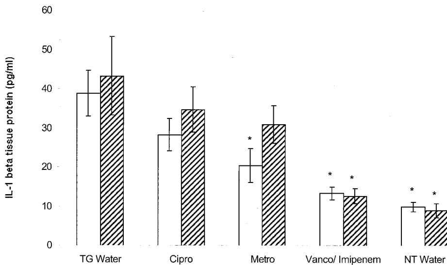
FIG. 3. Tissue IL-1 \beta protein concentrations of the ceca from B27 TG rats treated with different antibiotics starting before (4 weeks of age) ( \square ) and after (3 months of age) ( \text{▨} ) the onset of colitis. *, P < 0.05 versus TG water. Cipro, ciprofloxacin; Metro, metronidazole; Vanco, vancomycin. Error bars indicate SEMs.
