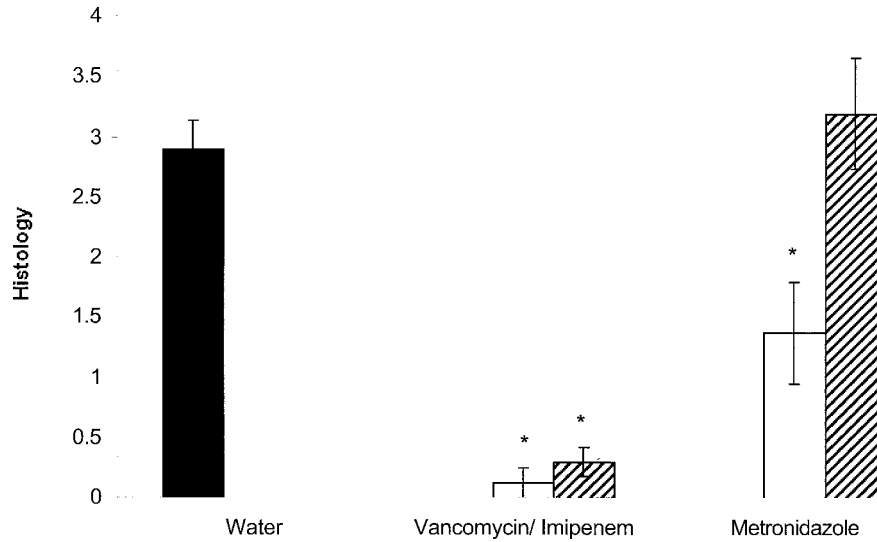
FIG. 4. Blinded histologic scores of the ceca from BALB/c mice with DSS-induced colitis treated with different antibiotics starting 3 days before or 2 days after the onset of DSS administration. The 5% DSS was continued for a total of 7 days. *, P < 0.05 versus water. □, Prevention; ▨, treatment; ■, water control. Error bars indicate SEMs.
