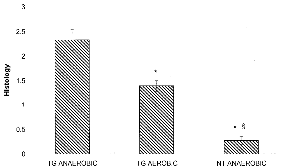
FIG. 7. Blinded histologic scores of the ceca from germfree B27 TG rats colonized for 1 month with cultures of SPF cecal bacteria incubated overnight under anaerobic or aerobic conditions. n = 6 to 9 rats/group. *, P < 0.05 versus anaerobic; §, P < 0.05 versus aerobic. Error bars indicate SEMs.
