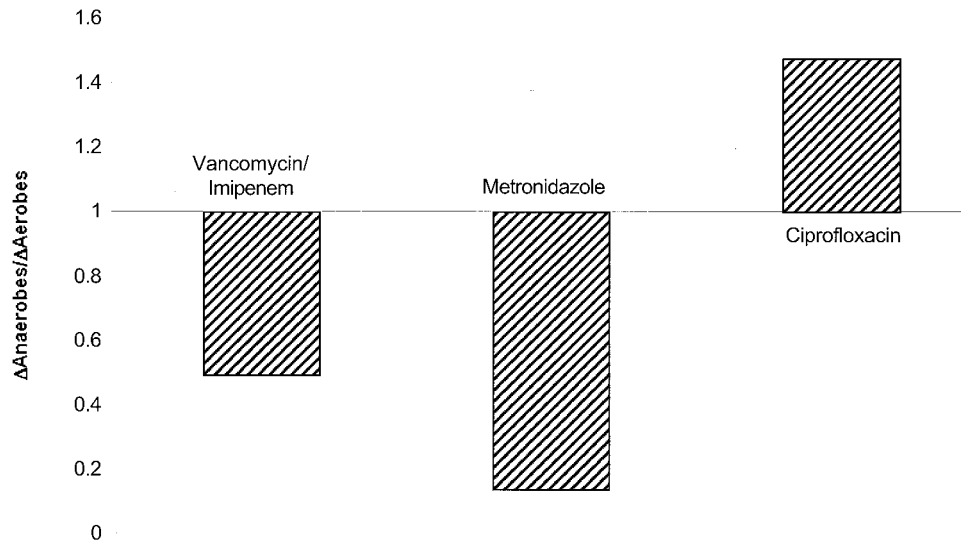
FIG. 6. Alteration of the ratio of anaerobic bacteria to aerobic bacteria by antibiotics compared to the ratio of anaerobic bacteria to aerobic bacteria in the water control group ( [\text{anaerobes/aerobes with antibiotics}]/[\text{anaerobes/aerobes for water control}] ). Antibiotic treatment resulted in an altered bacterial composition after 6 weeks. Compared with the water controls, vancomycin-imipenem reduced more anaerobes than aerobes as demonstrated by the decreased ratio of anaerobes to aerobes to 0.5 of that of the water control group. This alteration of bacterial composition was even exceeded by metronidazole, where the ratio of anaerobes to aerobes dropped to 1/10 of that of the water control group. In contrast ciprofloxacin reduced predominantly aerobes as shown by the increase of the anaerobic/aerobic ratio to 1.5-fold that of the water control group.
