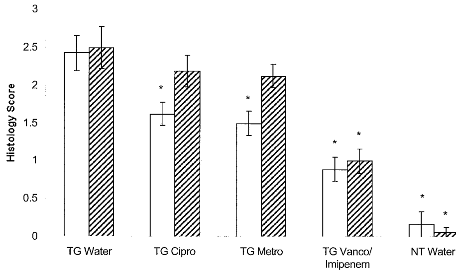
FIG. 1. Blinded histologic scores of the ceca from B27 TG treated with different antibiotics starting before (4 weeks of age, prevention protocol) (□) and after (3 months of age, treatment protocol) (▨) the onset of colitis. All rats were killed at 4 months of age. n = 8 or 9 rats in each group. *, P < 0.05 versus TG water controls. Cipro, ciprofloxacin; Metro, metronidazole; Vanco, vancomycin. Error bars indicate SEMs.
