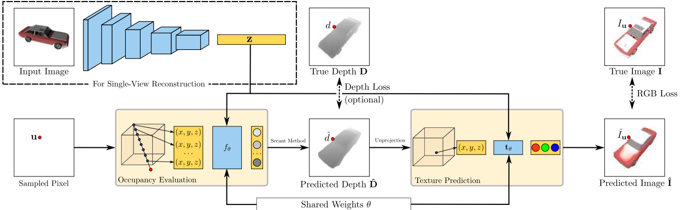
Figure 2: Differentiable Volumetric Rendering. We first predict the surface depth \hat{d} by performing occupancy evaluations for a given camera matrix. To this end, we project sampled pixel \mathbf{u} to 3D and evaluate the occupancy network at fixed steps on the ray cast from the camera origin towards this point. We then unproject the surface depth into 3D and evaluate the texture field at the given 3D location. The resulting 2D rendering \hat{\mathbf{I}} can be compared to the ground truth image. When we also have access to ground truth depth maps, we can define a loss directly on the predicted surface depth. We can make our model conditional by incorporating an additional image encoder that predicts a global descriptor \mathbf{z} of both shape and texture.
