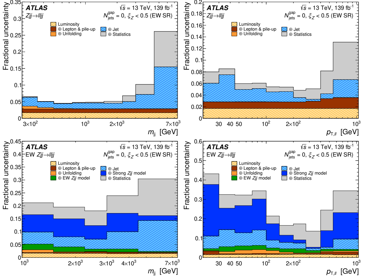
Figure 6: Fractional uncertainty in the inclusive Zjj measurement (top) and the EW Zjj measurement (bottom) as a function of m_{jj} (left) and p_{T, \ell\ell} (right). Uncertainty sources are grouped in categories that are added in quadrature (denoted \oplus ) to give the total uncertainty. The ‘EW Zjj model’ component includes the uncertainty on the EW Zjj prediction and the impact of interference between the strong Zjj and EW Zjj processes.
