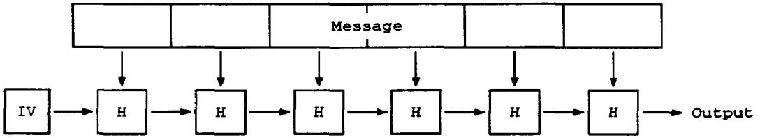
Figure 2: Outline of N-Hash
