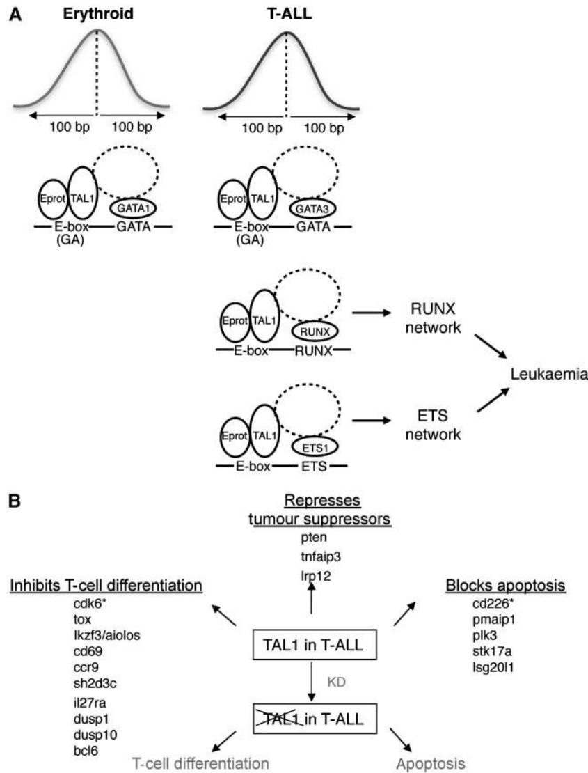
Figure 8 Model of TAL1-mediated leukaemogenesis. (A) TAL1 binds to different composite DNA motifs depending on the cellular environment. This alternate binding site selection provides TAL1 with access to RUNX and ETS transcriptional regulatory networks preferentially in T-ALL. Deregulation of transcriptional networks controlled by these important activators of T-cell differentiation could have a crucial role in the arrest of T-cell differentiation, potentially leading to T-cell leukaemia. (B) In the T-cell lineage, TAL1 inhibits tumour suppressors and mediators of differentiation and apoptosis. Upon TAL1 KD, T-ALL cells resume part of the T-cell transcriptional program and enter apoptosis. TAL1-regulated genes identified in our study, which could mediate these functions are indicated. All genes are repressed by TAL1, except those with an asterisk whose expression is increased by TAL1 in T-ALL.
