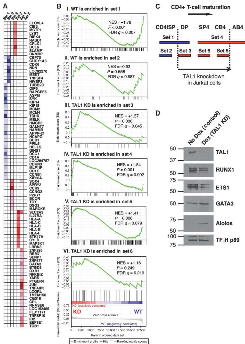
Figure 3 Jurkat cells are blocked at an immature stage resembling CD4 + intrathymic progenitors but partially re-enter the transcriptional program of T-cell differentiation upon TAL1 knockdown. (A–C) Gene set enrichment analysis (GSEA) was performed comparing microarray expression profiling of Jurkat cells upon TAL1 KD with signature gene sets established from expression profiling of purified normal primary human CD4 + T cells at different stages of differentiation (Lee et al , 2004). This analysis indicates that signature sets corresponding to early CD4 + intrathymic T-cell progenitors (sets 1 and 2) are enriched in the WT phenotype (in blue) while sets corresponding to more differentiated states (sets 3–6) are enriched in TAL1 KD phenotype (in red). For a detailed description of gene sets, see Supplementary data. (A) GSEA leading edge analysis heat map and list of enriched genes. (B) Enrichment plots for the six T-cell signature sets. NES, normalized enrichment score; FDR, false discovery rate. (C) Diagram summarizing the correlation between changes in gene expression profiles upon TAL1 KD in Jurkat cells and during CD4 + T-cell maturation. CD4ISP, CD4 immature single positive; DP, CD4 CD8 double positive; SP4, CD4 single positive; CB4, CD4 single positive from cord blood; AB4, CD4 single positive from adult blood. (D) TAL1 KD leads to profound changes in the protein levels of T-cell transcription factors. TAL1 KD was induced in Jurkat cells by the addition of Dox for 72 h. Nuclear extracts were prepared and analysed by western blot using antibodies indicated on the right. Molecular weight markers (in kDa) are indicated on the left.
