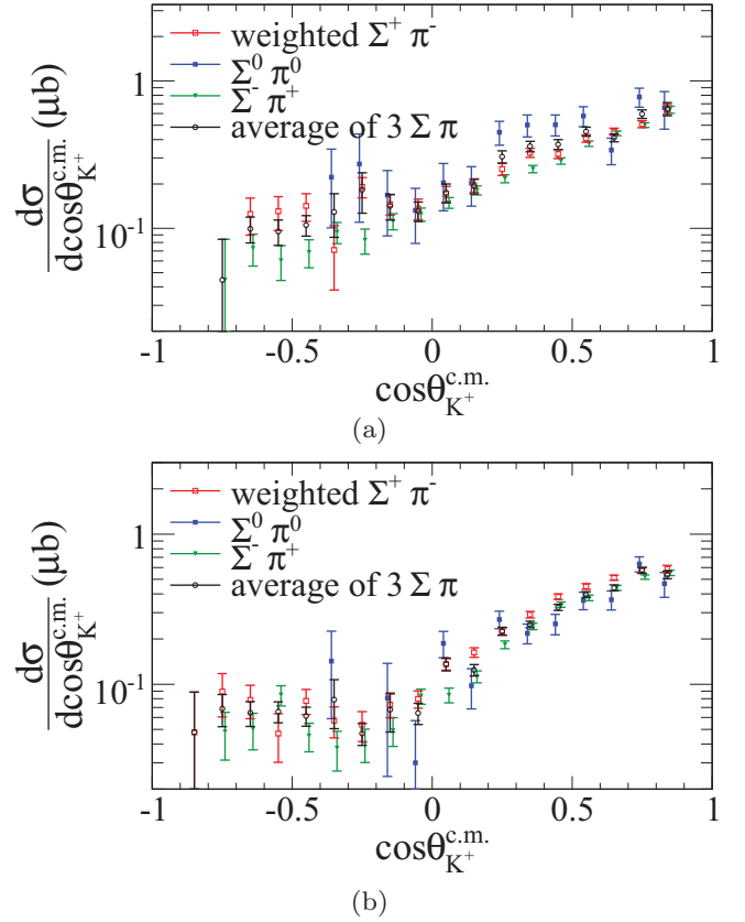
FIG. 8. (Color online) Comparison of the three \Sigma\pi decay modes for the \Lambda(1520) in two energy bins at 8(a) 2.05 \leq W \leq 2.15 GeV and 8(b) 2.45 \leq W \leq 2.55 GeV as a function of center-of-mass kaon angle. For clarity, the data have been shifted slightly to prevent overlaps.
