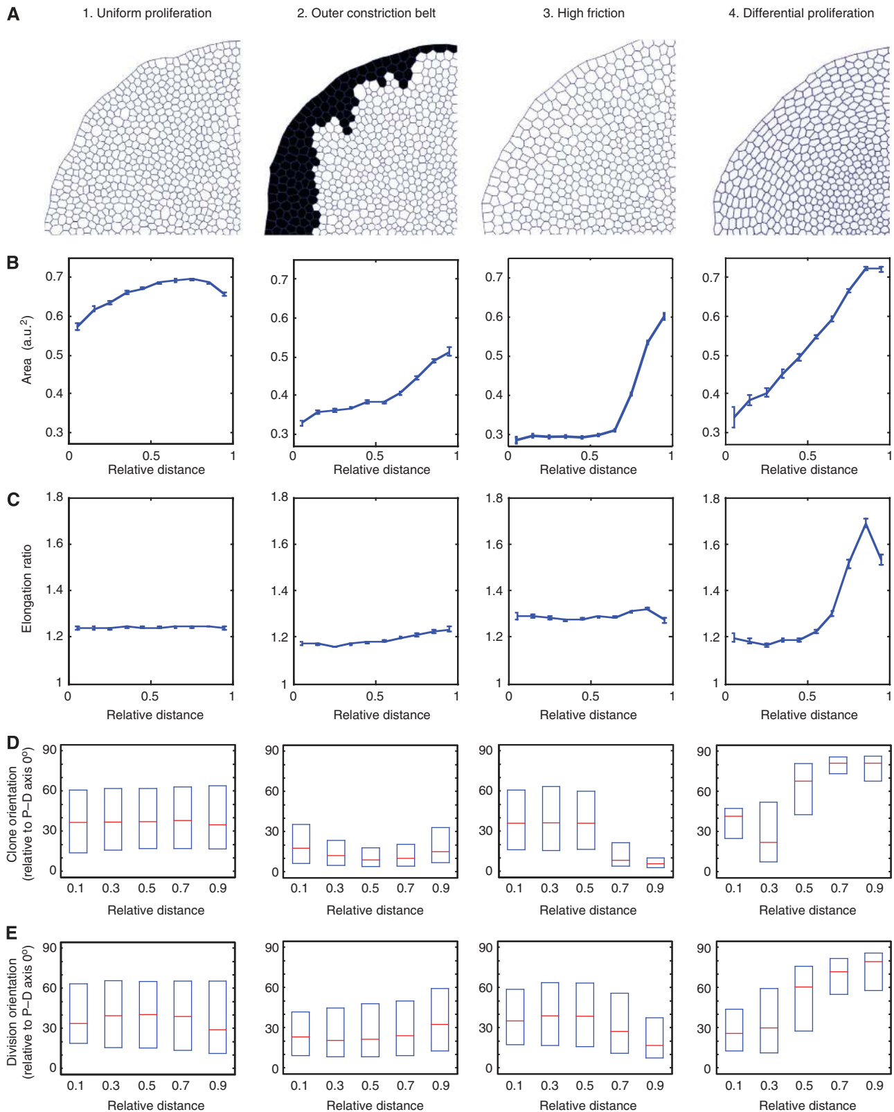
Figure 5 Computational exploration of the different mechanisms that can generate global forces to elongate cells in the periphery of the disc. A radial (P–D) polarization of Dach5 is applied to all simulations to mimic the in vivo Dach5 polarization patterns. (A) Snapshots of a quadrant of the in silico wing discs after ‘60 h real time’ simulations (equivalent to between 2 and 10 h computational run time, depending on scenario). (B–E) All graphs show relative distance from the centre of the disc on the X axis. (B) Cell area (arbitrary units) at end point. Error bars represent s.e.m. (C) Cell elongation ratios at end point. Error bars represent s.e.m. (D) Clones are induced in silico and their elongation orientations (relative to the radial P–D axis) are recorded at end point. Plots show median and first and third quartiles. Note the baseline bias of orientations towards the P–D axis, due to Dach5. (E) Cell division orientations are tracked throughout the run. Showing median and first and third quartiles. See Supplementary Figure S6 for detailed analysis of cell elongation orientations. The profile of the steep differential proliferation in mechanism (4) is shown in Supplementary Figure S6D, top panel.
