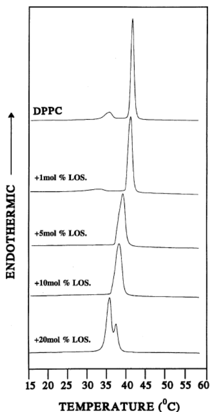
Figure 7: Normalized DSC scans of DPPC bilayers containing losartan at different concentrations (Adapted from Fig.2 of ref [79] )
