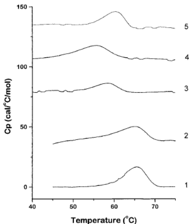
Figure 4: DSC heating curves for the thermal denaturation of GLUT 1. Curve 1, No addition; curve 2, in the presence of 0.4 M NaCl; curve 3, in the presence of 4.8 mM ATP and 0.4 M NaCl; curve 4, in the presence of 4.8 mM ATP; curve 5, in the presence of 4.8mM ATP and 500mM D-glucose (Adapted from Fig.3 of ref [70] )
