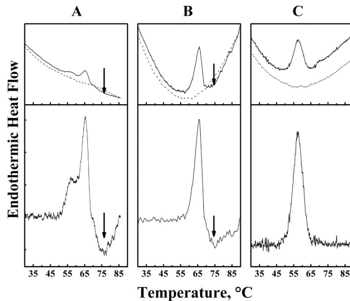
Figure 2: DSC thermograms observed during the thermal unfolding of S. lividans xylanase A. The data are representative of the intact enzyme (A), the catalytic domain (B), and the xylan binding domain (C). The top panels show thermograms observed during the unfolding of the protein (solid lines) and those obtained in subsequent heating scans after complete suppression of all protein-related thermotropic events (broken line). The bottom panels show the unfolding thermograms after baseline subtraction. (Adapted from Fig.1 of ref [38] )
