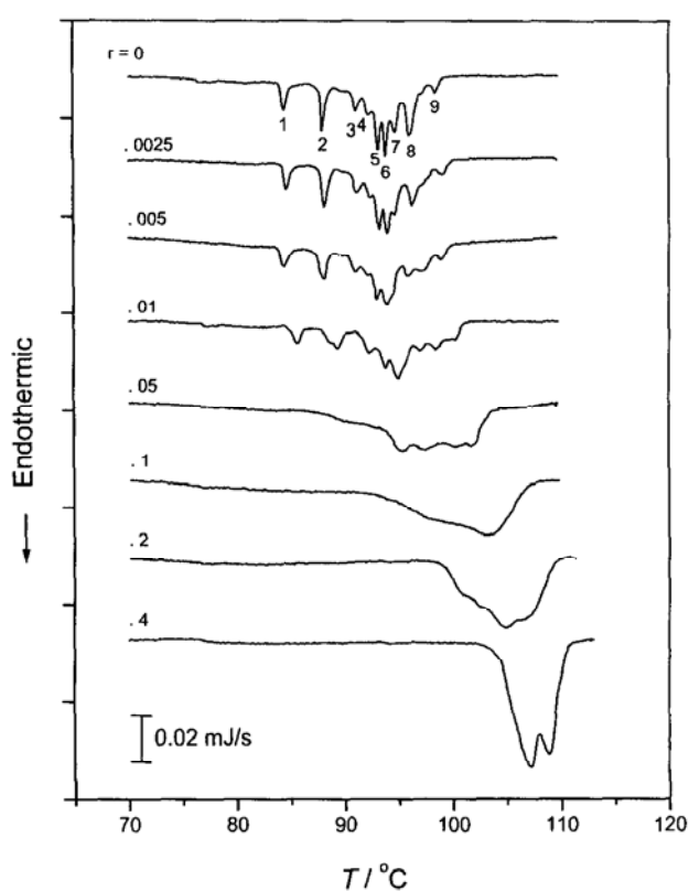
Figure 8: DSC curves of ColE1 plasmid DNA in solutions of various distamycin concentrations. Distamycin concentration was indicated as r, the molar ratio of distamycin to base pairs of DNA (Adapted from Fig.3 of ref [88] )
