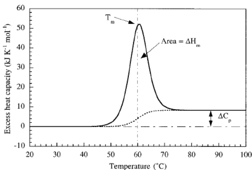
Figure 1: DSC experiment for the two-state unfolding of a globular protein (Adapted from Fig.1 of ref [1] )
