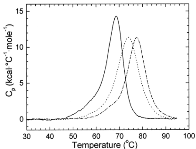
Figure 9: DSC thermograms for the d(TGCT)·d(AGCA) unplatinated duplex ( solid line ) containing a single, site-specific interstrand cross-link of cisplatin ( dot-dash line ) or transplatin ( dashed line ). (Adapted from Fig.2 of ref [92] )
