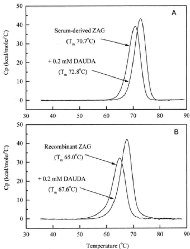
Figure 5: Increased thermal stability of ZAG upon ligand binding. Normalized DSC data, corrected for buffer base line showing cooperative endothermic unfolding of wild-type (A) and recombinant ZAG (B) in the presence and absence of 0.2 mM DAUDA. (Adapted from Fig.4 of ref [72] )
