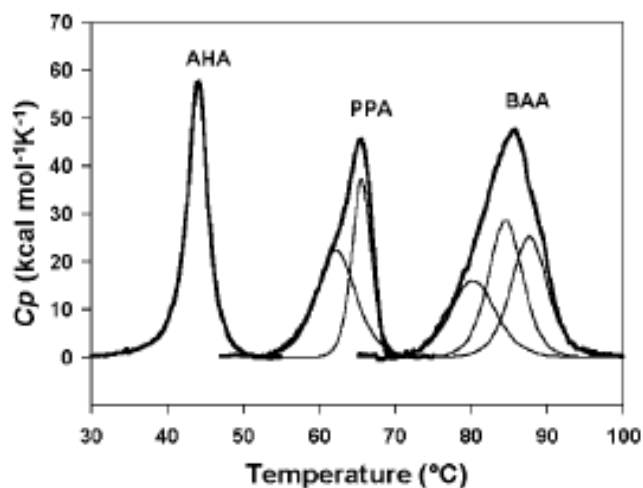
Figure 3: Thermal unfolding of \alpha -amylase recorded by DSC. AHA: psychrophilic \alpha -amylase from P. haloplanktis ; PPA: pig pancreatic \alpha -amylase; BBA: Bacillus amyloliquefaciens \alpha -amylase. Deconvolution shows two and three calorimetric domains for PPA and BAA respectively (Adapted from Fig.1 of ref [47] )
