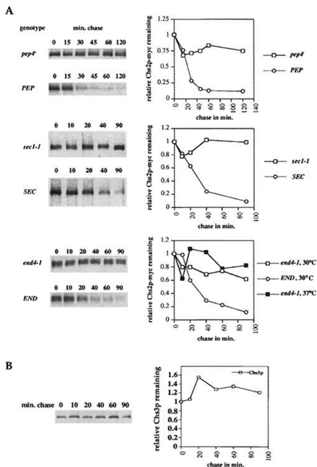
Figure 6. Chs2p-myc, in contrast with Chs3p, is rapidly degraded in a PEP4 -, SEC1 -, and END4 -dependent manner. Cells were labeled for 10 min with 35 S-Pro-mix, chased for the indicated times, lysed, and immunoprecipitated for Chs2p-myc (A) or Chs3p (B). (A, top panel) Strains JCY380 ( PEP CHS2MYC ) and JCY381 ( pep4 - CHS2MYC ) were grown and kept at 30°C throughout the course of the experiment. (A, middle panel) Strains JCY396 ( sec1-1 CHS2MYC ) and JCY397 ( SEC CHS2MYC ) were grown at 25°C, and then preincubated for 45 min, labeled, and chased at 37°C. (A, bottom panel) Strains JCY389 ( end4-1 CHS2MYC ) and JCY390 ( END CHS2MYC ) were grown at 25°C, and then preincubated for 45 min, labeled, and chased at 30°C. Quantification of Chs2p-myc stability in end4-1 at 37°C is also shown in the graph (A, bottom right). (B) JCY380 was grown, labeled, chased at 30°C, and then immunoprecipitated with anti-Chs3p Abs.
