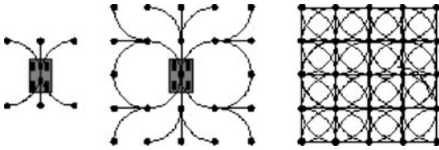
Figure 2. A 3D search space, consisting of position and heading (x, y, \theta) . The Reeds–Shepp car can move forward and backward. It can drive straight or turn left or right at a fixed curvature. Left: The designed control set precisely hits vertices in a rectangular grid. It was derived from the car’s basic motions by carefully choosing their length. Center: The reachability tree to depth 2. Right: The reachability tree (search space) obtained by copying the control set at every vertex in a C space with four headings. Each dot represents four distinct vertices overlaid on each other, each representing different values of heading. Although this search space will not generate a turn of less than the chosen curvature, and although heading is continuous across vertices, the instantaneous transitions of curvature at the vertices do not respect steering rate limitations. Moreover, considering only four different heading values typically is impractical.
