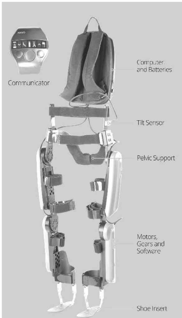
Fig. 1. The basic configuration of the ReWalk device.
