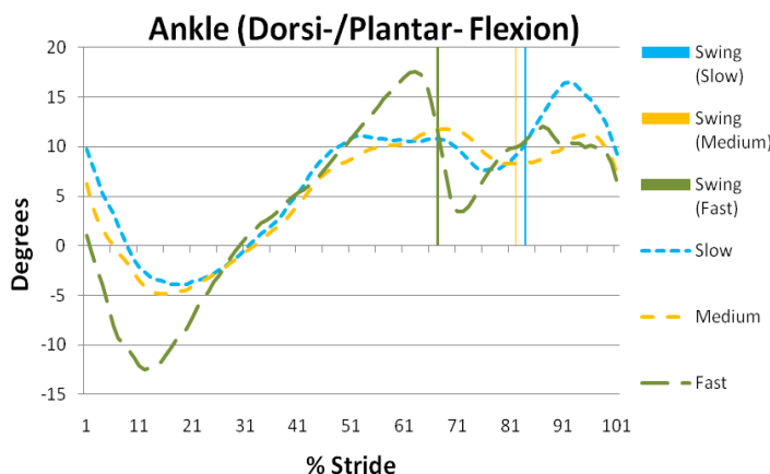
Fig. 5. Ankle plantarflexion and dorsiflexion for all three groups. Vertical lines demarcate the start of swing phase.
