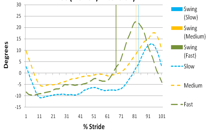
Fig. 4. Knee flexion/extension for the three groups. Data were time normalized. The solid vertical lines demarcate the start of swing phase.
