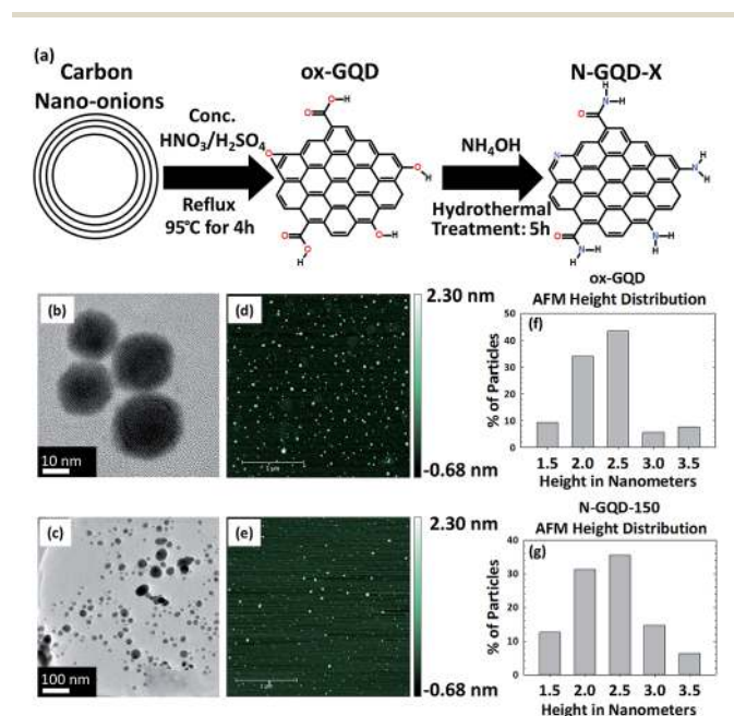
Fig. 1 (a) A scheme for the synthesis of GQDs and N-GQDs. TEM images of ox-GQD (b) and N-GQD (c), AFM images of ox-GQD (d) and N-GQD (e), and the histogram of the thickness of ox-GQDs (f) and N-GQDs (g).
