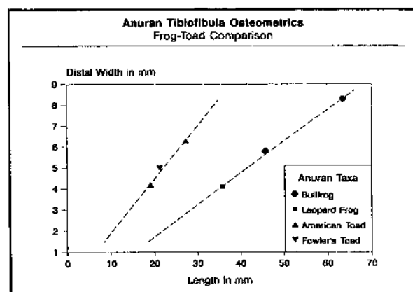
Figure 6. Shaft length & distal width measurements for tibiofibulae from species in the general Rana & Bufo . Broken lines indicate approximate trends in length:width ratios.
