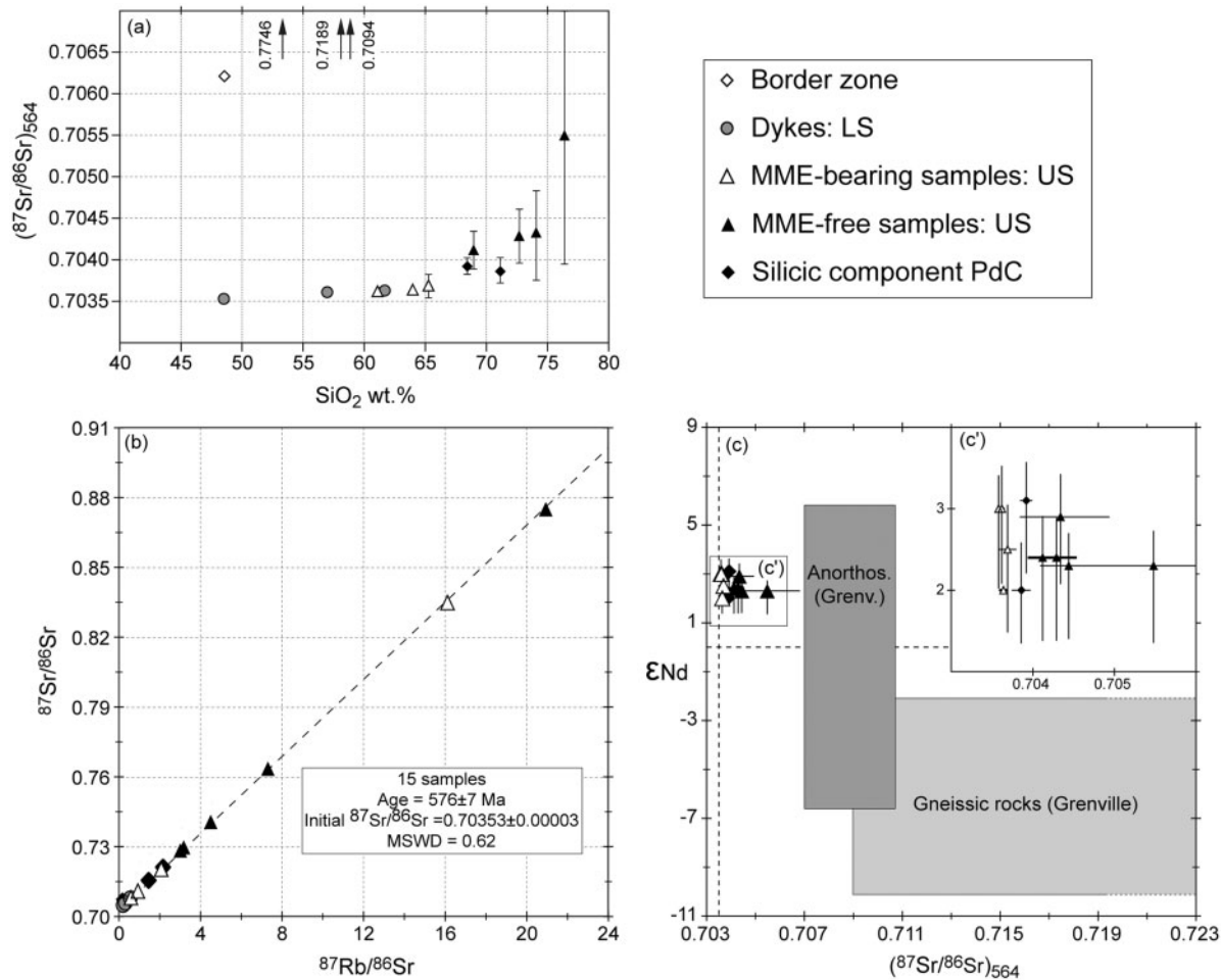
Fig. 12. (a) Initial Sr-isotopic ratios (calculated at 564 Ma) vs SiO 2 (wt %). Arrows are directed toward the isotopic compositions (given values) of country-rock samples. (b) Rb–Sr isochron of Sept Iles fine-grained and silicic samples (calculated at 564 Ma). The compositions of the country-rocks in the area of Sept Iles are also indicated (data from Wadleigh et al. , 1985; Ashwal et al. , 1986; Shaw et al. , 1986; Dickin & Higgins, 1992; Olive et al. , 1997; Dickin, 2000). (c') Close-up of variation in Sept Iles samples. Error bars for Sr and Nd isotopic ratios were calculated using expected errors in the determination of Rb ( \pm 5\% ), Sr ( \pm 2\% ), Sm and Nd ( \pm 5\% ; Vander Auwera et al. , 1998a).
