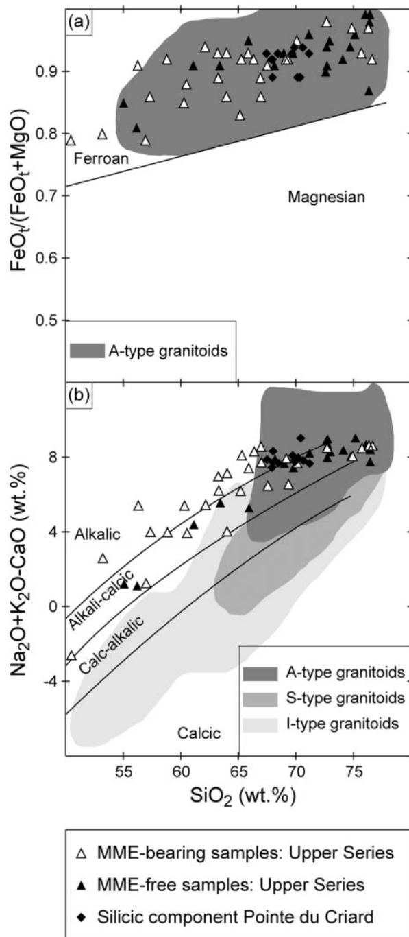
Fig. 7. Major element geochemical characteristics of silicic samples from the Upper Series and the Pointe du Criard sill. (a) \text{FeO}_t/(\text{FeO}_t + \text{MgO}) vs \text{SiO}_2 (wt %) discriminant diagram of Frost et al. (2001). (b) \text{Na}_2\text{O} + \text{K}_2\text{O} - \text{CaO} (wt %) vs \text{SiO}_2 (wt %) discriminant diagram of Frost et al. (2001).
