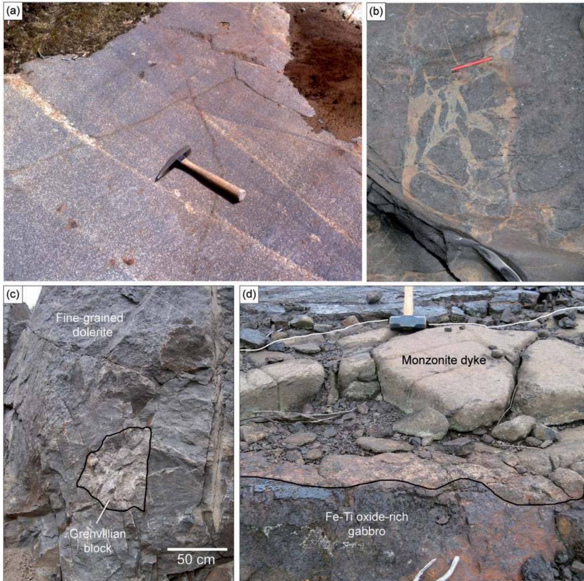
Fig. 3. Field relations in the Sept Iles layered intrusion. (a) Representative outcrop of the Layered Series showing decimetre-scale modal layering with an erosive channel in gabbroic rocks. (b) Matrix of silicic material invading anorthosite fragments from the Upper Border Series. Pen is 13 cm long. (c) Quartzite block from the country-rocks enclosed in fine-grained dolerite in the Border Zone. (d) Metre-scale dyke of intermediate (monzonite) composition cross-cutting Fe–Ti oxide-rich gabbros of the Layered Series.
