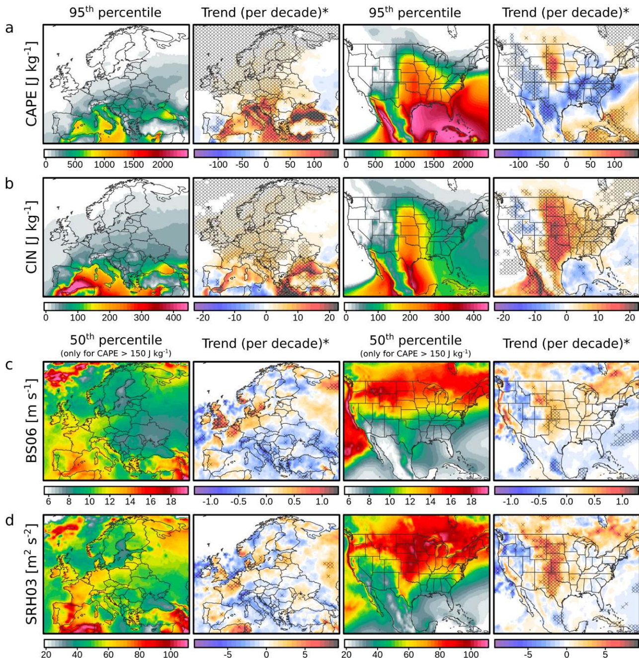
Fig. 2. As in Fig. 1, but for the 95th percentile of (a) convective available potential energy (CAPE), (b) absolute value of convective inhibition (CIN), and (c) 50th percentile of vertical wind shear (BS06) and (d) storm-relative helicity (SRH03). For BS06 and SRH03 only situations with \text{CAPE} > 150\text{ J kg}^{-1} are considered.
