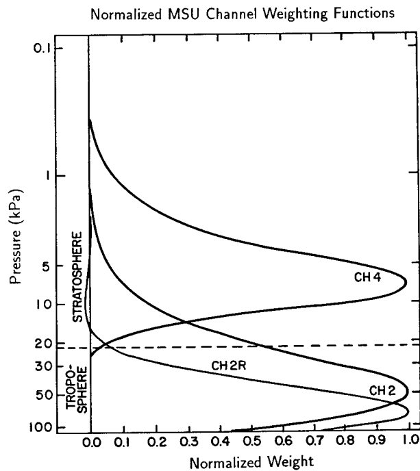
FIG. 1. Normalized weighting functions for MSU channels 2 (53.74 GHz), 4 (57.95 GHz), and MSU 2R for a 22^\circ view angle through a U.S. Standard Atmosphere . The dashed line represents the level of the tropopause.
