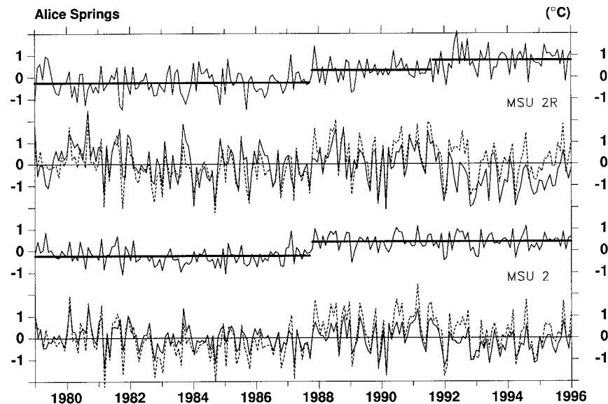
FIG. 8. Monthly mean temperature anomalies from MSU (solid) and Alice Springs (dashed), and the differences (Alice Springs minus MSU), for MSU 2R (upper two curves) and MSU 2 (lower two curves). Also indicated are the mean differences (heavy) before and after August 1987 for MSU 2, as well as before and after June 1991 for MSU 2R. The anomalies are relative to the 1982–91 means.
