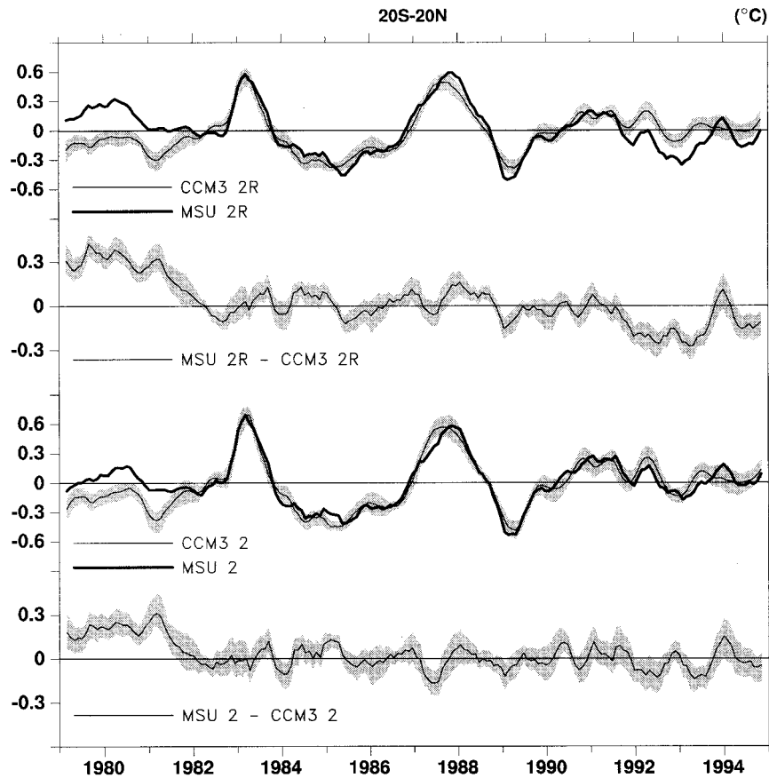
FIG. 7. Five-month running mean MSU channel 2 and 2R temperature anomalies (heavy solid) and the five-member ensemble mean equivalent MSU anomalies from CCM3 integrations (thin solid) and the range about the means (stippled) area-averaged over the Tropics (20°S–20°N). Also shown are the differences (MSU – CCM) for MSU 2R (top) and MSU channel 2 (bottom).
