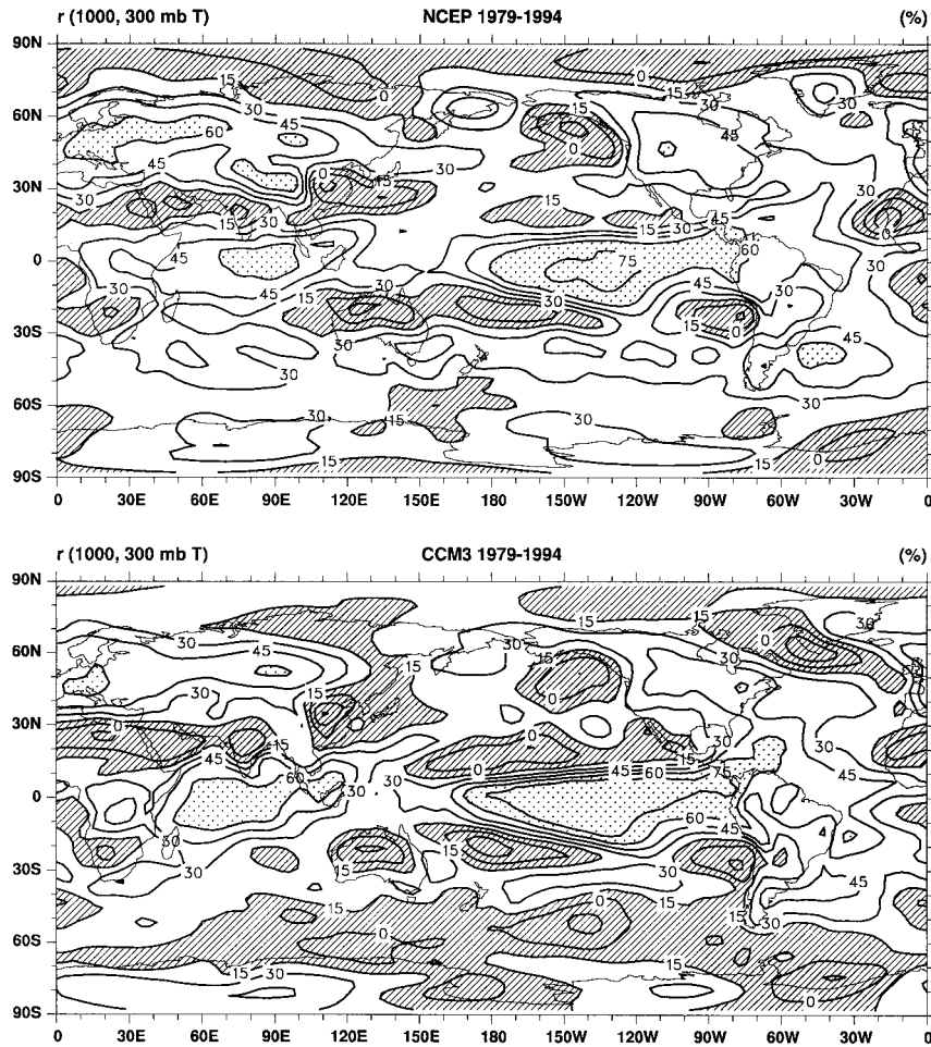
FIG. A2. Correlation coefficients (%) over 192 months between 1000- and 300-mb temperature anomalies from (top) the NCEP reanalyses and (bottom) three-member ensemble mean anomalies from CCM3 integrations forced with observed global SSTs. Monthly anomalies were computed relative to the mean annual cycle for 1982–91. Values less than 15% are hatched and values greater than 60% are stippled.
