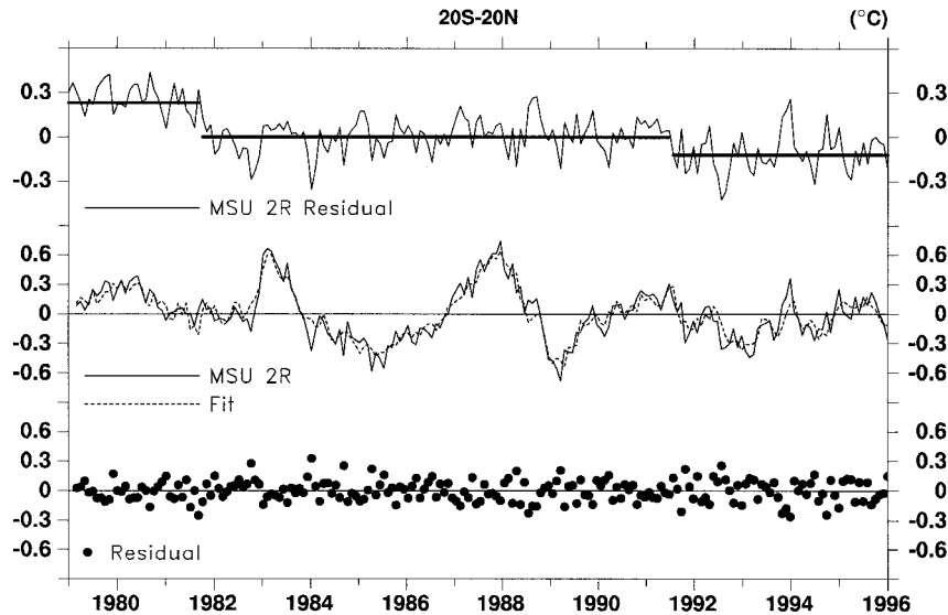
FIG. 11. (Top) Monthly MSU 2R residuals after removing the SST effects through linear regression, as in Fig. 4, and the means of the residuals determined before and after the two breakpoints identified by an objective change-point analysis technique (heavy lines); (middle) monthly MSU 2R anomalies (solid) with fitted values (dashed); (bottom) residuals obtained from the linear model described in the text.
