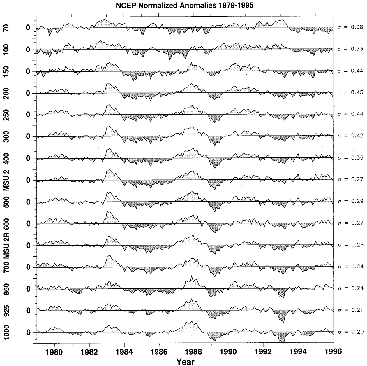
FIG. 9. Normalized tropical (20°S–20°N) temperature anomalies relative to the 1979–95 means of NCEP reanalyzed temperatures at pressure levels from 1000 to 70 mb. The standard deviations ( ^{\circ}\text{C} ) of the monthly anomalies are given on the right axis, and the tick marks on the left axis are every 3\sigma . The observed MSU 2R and MSU channel 2 normalized anomalies are also provided near the pressure levels of the peaks in their respective weighting functions. Negative anomalies are given by the darker shading.
