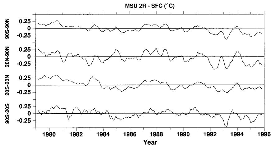
FIG. 2. Five-month running mean differences ( ^{\circ}\text{C} ), MSU 2R minus surface temperature anomalies, relative to the 1982–91 means averaged over the globe ( 90^{\circ}\text{S} – 90^{\circ}\text{N} ), the Northern Hemisphere extratropics ( 20^{\circ} – 90^{\circ}\text{N} ), the Tropics ( 20^{\circ}\text{S} – 20^{\circ}\text{N} ), and the Southern Hemisphere extratropics ( 20^{\circ} – 90^{\circ}\text{S} ).
