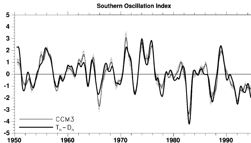
FIG. A1. Observed (heavy solid) and the five-member ensemble mean (thin solid) equivalent Southern Oscillation index from CCM3 integrations and the range about the means (stippled). The values were smoothed with a low-pass 11-term filter that eliminates fluctuations of less than 8 months but retains periods exceeding 24 months (Trenberth 1984).
