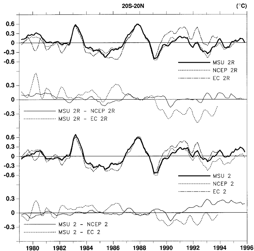
FIG. 10. Five-month running mean MSU channel 2 and 2R temperature anomalies (solid) and the equivalent anomalies from the NCEP (dashed) and ECWMF (dash-dot) reanalyses area-averaged over the Tropics ( 20^{\circ}\text{S} – 20^{\circ}\text{N} ). Also shown are the differences (MSU – NCEP) and (MSU – ECWMF) for MSU 2R (top) and MSU channel 2 (bottom).
