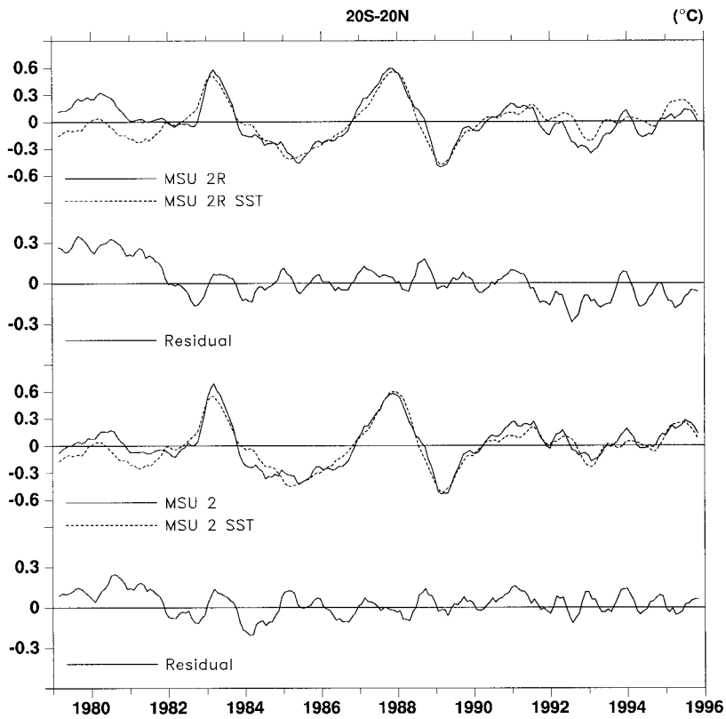
FIG. 4. Five-month running mean MSU channel 2 and 2R temperature anomalies area-averaged over the Tropics (20°S–20°N). The dashed lines represent the MSU anomalies associated with SST variations (leading by one month) from linear regression over the period 1982–91. Also shown are the residuals after removing the linear SST effects for MSU 2R (top) and MSU channel 2 (bottom).
