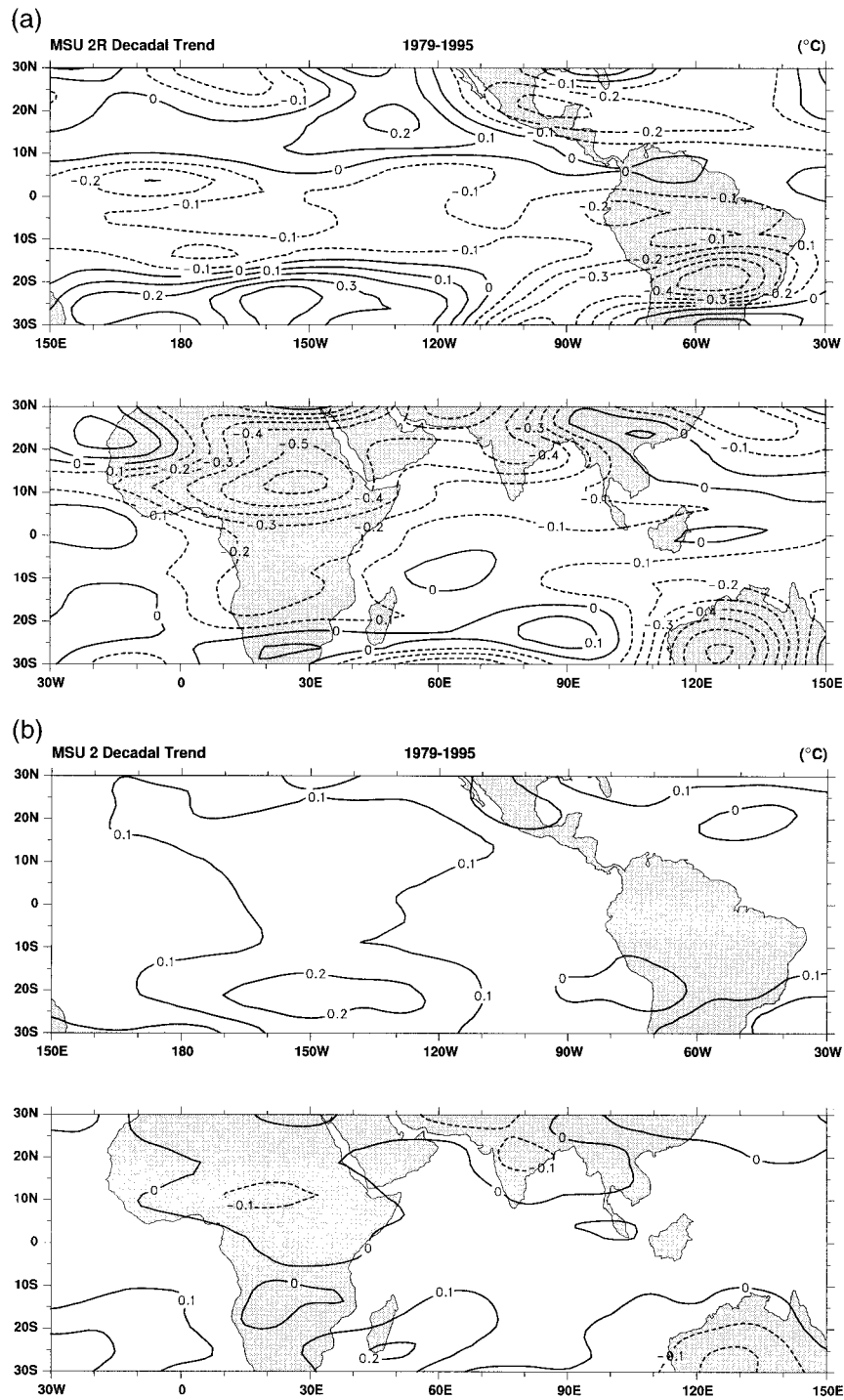
FIG. 6. Linear trends ( ^{\circ}\text{C decade}^{-1} ) in (a) MSU 2R temperatures and (b) MSU channel 2 temperatures computed from monthly anomalies over the period 1979–95. Negative trends are dashed, and the contour increment is 0.1^{\circ}\text{C decade}^{-1} .
