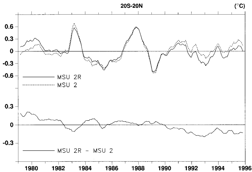
FIG. 5. Five-month running mean MSU channel 2 and 2R temperature anomalies, and the differences (MSU 2R – MSU 2), area-averaged over the Tropics (20°S–20°N). The anomalies are relative to the 1982–91 means.
