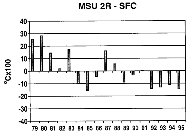
FIG. 3. Tropical ( 20^{\circ}\text{S} – 20^{\circ}\text{N} ) annual mean temperature anomaly differences ( \times 100^{\circ}\text{C} ), MSU 2R minus surface, relative to the 1982–91 means.
