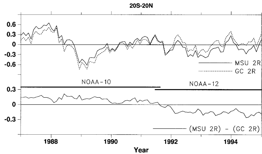
FIG. 14. (Top) Monthly anomalies from Christy et al. (1995) (MSU 2R) and from Goldberg and Crosby (1995) (GC 2R) relative to the 1987-94 means, and (bottom) their difference ( \text{C} ), MSU 2R - GC 2R. Also indicated are the periods of operation for NOAA-10 and NOAA-12.
