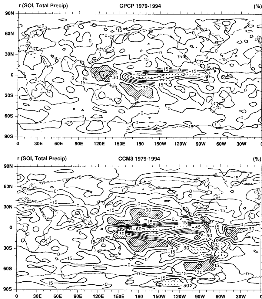
FIG. A3. Correlation coefficients (%) over 192 months between the observed Southern Oscillation index (as defined in the text) and (top) total precipitation from the Global Precipitation Climatology Project (see Xie and Arkin 1996) and (bottom) three-member ensemble mean anomalies from CCM3 integrations forced with observed global SSTs. Values less than -30\% are stippled and values greater than 30\% are hatched.
