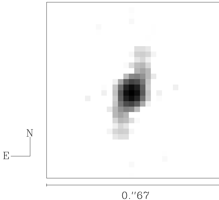
FIG. 1.—Nucleus of NGC 1068 at 0''.05 (3.6 pc) resolution. Pixels are 0''.021 on a side, and the field of view has been clipped to 0''.67 square. The image is shown in a logarithmic stretch and is comprised of two components—a point source containing 49% of the total nuclear flux and an extended component lying at a position angle of 159° and containing 51% of the total nuclear flux.
