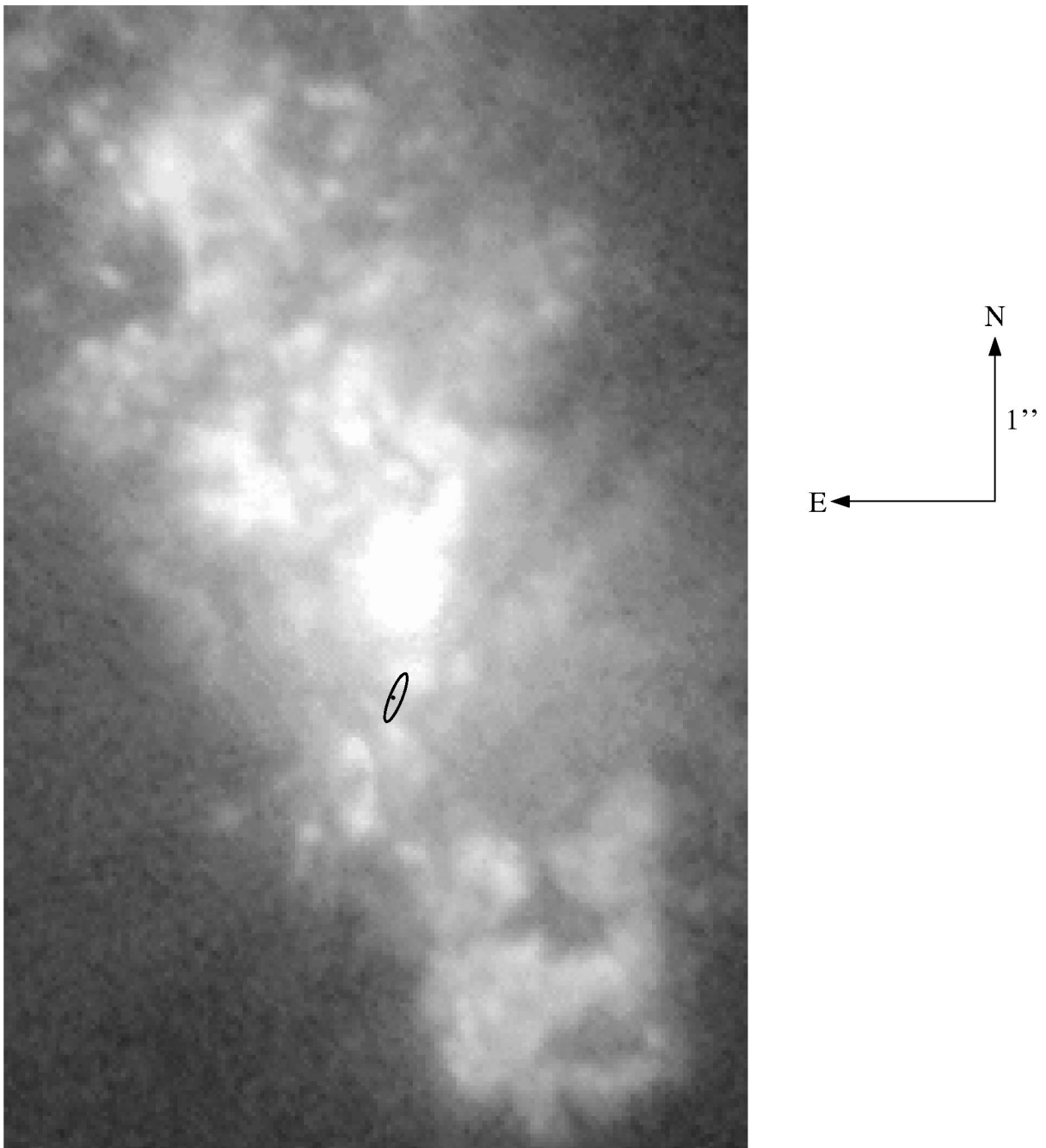
FIG. 5.—Location and size of the extended K -band emission ( ellipse ), superposed with the HST [O\ III] emission line image of Macchetto et al. (1994). The infrared point source was located at the center of polarization determined by Capetti et al. (1995). The K -band flux does not arise from any of the bright clumps of material that produce the narrow lines.
