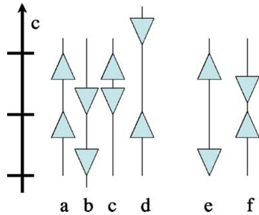
Fig. 3 Combination patterns of \text{CO}_3 – \text{CO}_3 pair in the A site. Triangles represent \text{CO}_3^{2-} with one of three C–O bonds of \text{CO}_3 laying on the c -axis. Note that existence of pattern (e) or (f) is implausible
