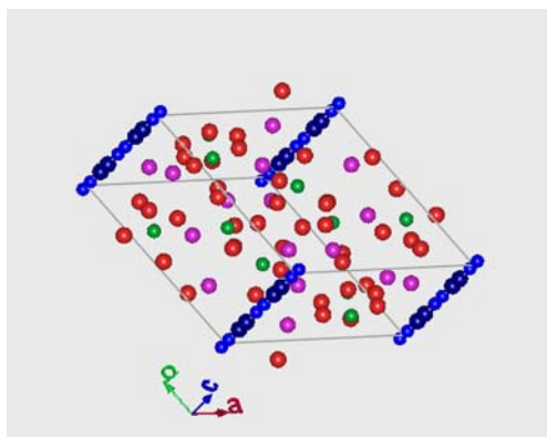
Fig. 2 Spatial repartition of the different atoms in the case of HAP. Hydrogen and oxygen atoms of the hydroxyl groups represented in blue are located on the c -axis
