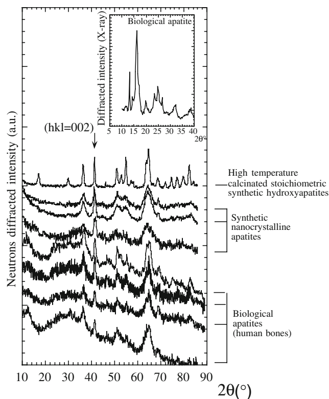
Fig. 5 Neutron diffraction diagrams of three families of apatite: high-temperature-calcinated synthetic apatite, room-temperature synthetic apatites and biological apatites (bones). In the insert , an X-ray diffraction diagram is visualised
