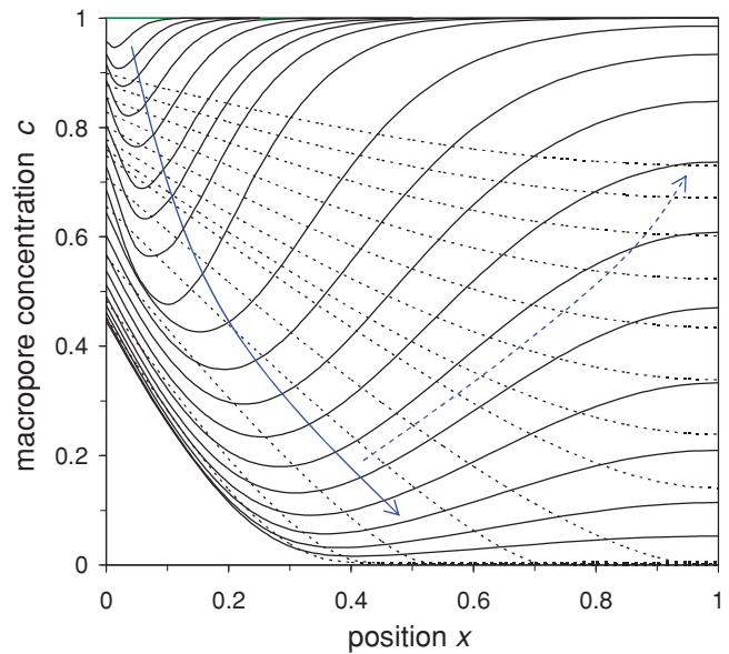
FIG. 9. (Color online) Macropore concentration profiles within the electrode as a function of time using the mD model. Starting at concentrations c = 1 , after applying a voltage of \phi_1 = 20 , first a local dip in concentration develops which flattens out (solid lines and arrow), while concentrations deep within the electrode reach a minimum ( t \sim 0.8 ), after which the salt concentration in the macropores slowly increases again (dashed lines and arrow).
