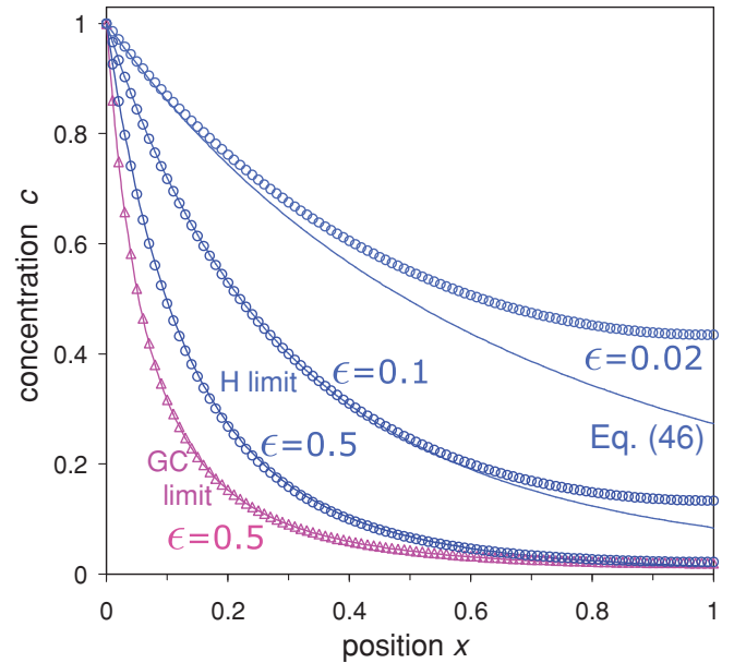
FIG. 5. (Color online) Steady-state profiles of salt concentration in the porous electrode for different values of the ratio \epsilon of the Debye length to the mean pore size. Comparison of analytical results [Eqs. (44) and (46)] with full numerical calculations [Eqs. (39) and (40)] in the GC limit (pink line, triangles) and H limit (blue lines, bullets). Transport in the stagnant diffusion layer is assumed to be fast ( \text{Bi} = \infty ), and other parameter values are \eta^0 = -10 ; k_R = j_O = 0.033 (GC limit) or k_R = j_O = 1 (H limit).
