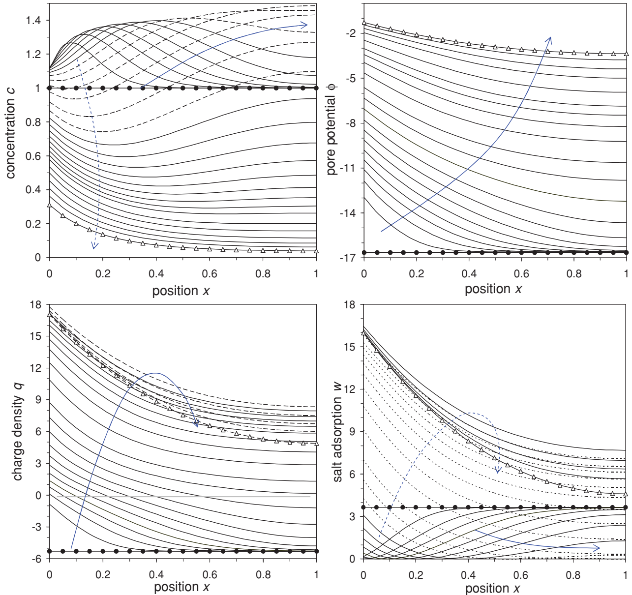
FIG. 7. (Color online) Numerical results for the profiles of salt concentration c , pore potential \phi , diffuse layer charge density q , and salt adsorption w in the electrode as a function of time (direction of arrow, first solid then dashed, and finally solid, 0.001 < t < 3 ). Filled circles denote the initial condition, and open triangles denote the steady state. The applied voltage (relative to solution) is \phi_1 = -12 , \delta = 0.23 , k_R = 0.033 , and j_O/k_R = 0.01 , i.e., \Delta\phi^{\text{eq},0} = \ln(k_R/j_O) \sim 4.6 . With these settings, the DLs are initially negatively charged and then eventually become positively charged after the voltage is applied. This sign reversal, coupled to nonlinear dynamics of ion transport at two different time scales (for capacitive and Faradaic charging) leads to the complicated nonmonotonic transient seen in the figure. A movie of this simulation is available as supporting online material [81].
