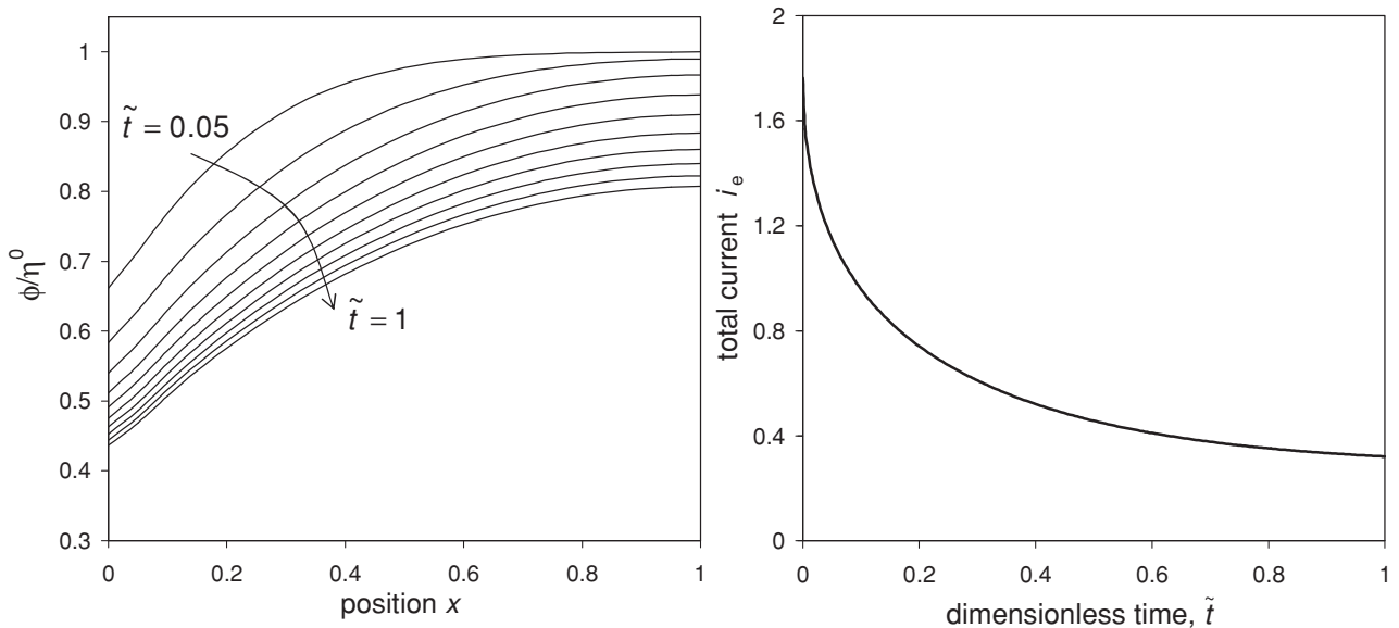
FIG. 3. Early time dynamics in response to a small applied voltage. (a) Evolution of the pore potential as function of position in the electrode as predicted by Eq. (32) for Bi = 2 and Da = 2 at different values of the dimensionless time \tilde{t} . (b) Total current development predicted by Eq. (33) ( Bi = 2 and Da = 2 ) when a small voltage ( \phi_1 = -1 ) is applied.
