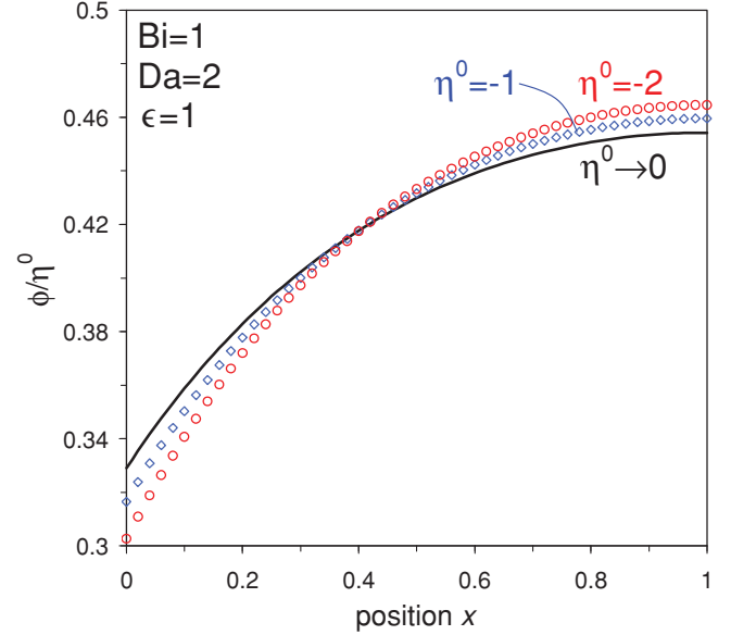
FIG. 4. (Color online) Steady-state pore potential \phi (scaled to \eta^0 ) as a function of position in the electrode according to Eq. (40) (bullets, H limit, no further assumptions) and according to Eq. (42) (solid line, both GC and H limits, linearized, i.e., pore concentration c \sim 1 ). For sufficiently small values of \phi_1 , all steady-state curves will collapse onto the limiting curve (solid line), Eq. (42).
