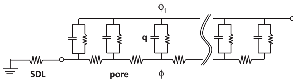
FIG. 2. Equivalent circuit ( RC transmission line [80]) for the linear response of the porous electrode in our model including both capacitive charging and Faradaic reactions. The quasineutral solution in the macropores acts as a series of resistors coupled to the electrode by parallel elements, each of which consists of two parallel elements, namely, a charge-transfer resistance and a DL capacitance (consisting of the diffuse and Stern layer differential capacitances in series [54]).
