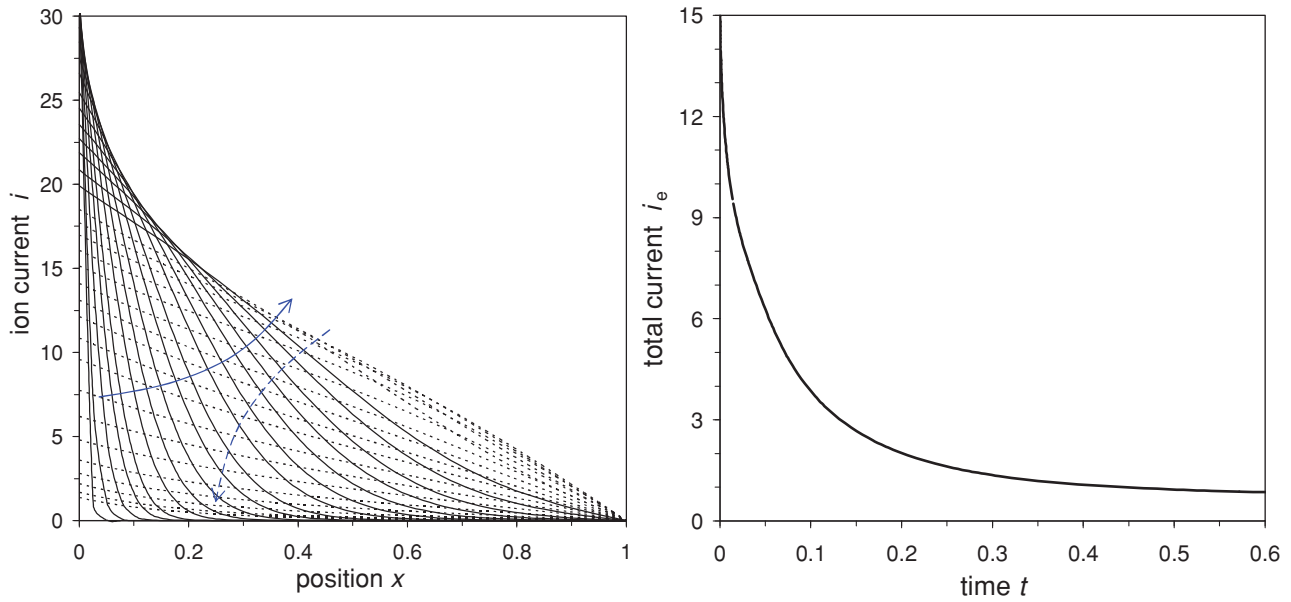
FIG. 8. (Color online) (a) Ion current profiles in the electrode as a function of time. Arrows show the direction of time, solid curves for 0.001 < t < 0.015 , dashed curves for 0.015 < t < 0.6 . Ion current at position x = 0 equals the total current i_e . (b) Total current i_e versus time t .
