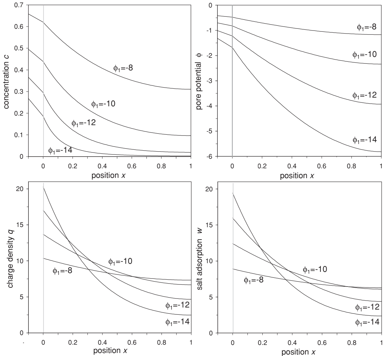
FIG. 6. Numerical results for the steady-state profiles of salt concentration c , pore potential \phi , diffuse-layer charge density q , and salt adsorption w in the electrode as a function of the applied potential \phi_1 ( k_R = j_0 = 0.033 ; \delta = 0.23 ). For these kinetic rate constants, the electrode is uncharged at equilibrium (i.e., \Delta\phi^{eq,0} = 0 ).
