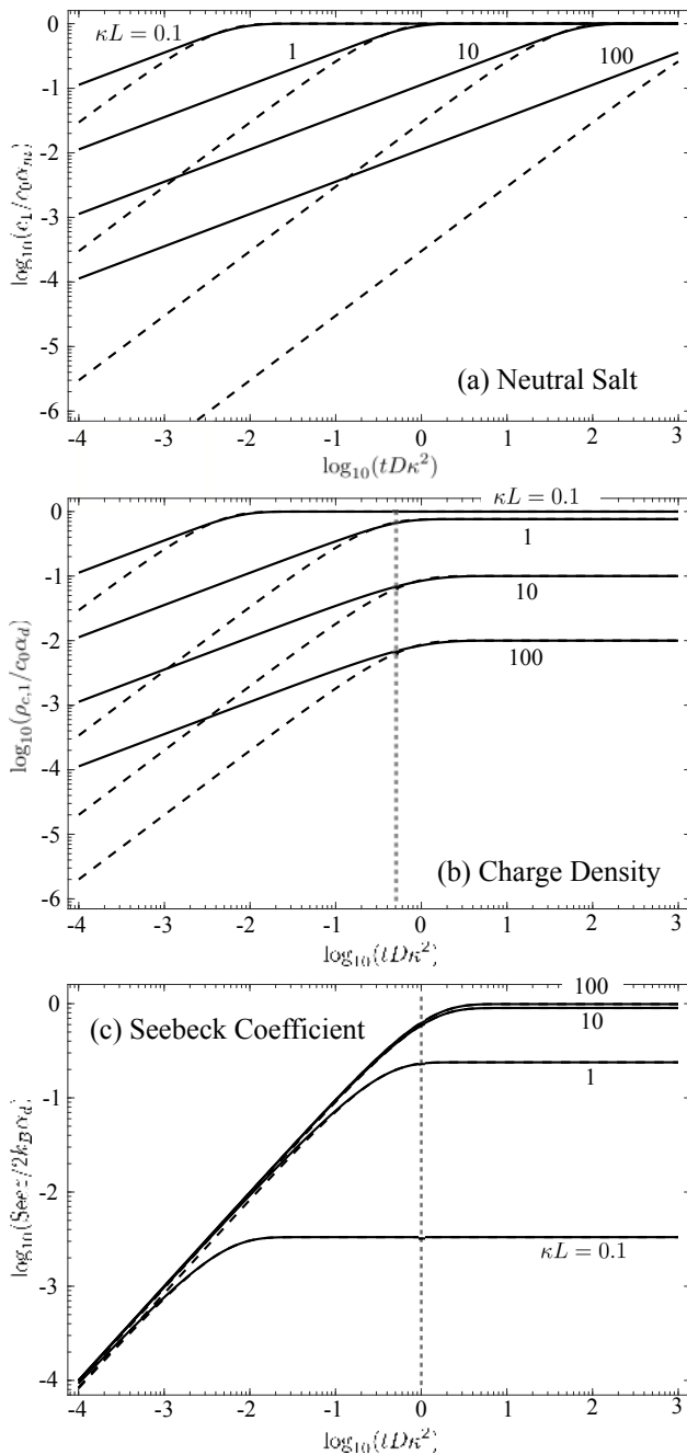
FIG. 3: Salt concentration (a) and charge density (b) at the cold electrode ( x = -L ) along with the Seebeck coefficient (c), \text{Se}(t) = -V(t)/\Delta T , versus time at \kappa L = 0.1, 1, 10 and 100 . Numerical Laplace transform inversion of (20) are shown as solid lines; dashed lines are the long time solutions (22). The salt concentration increases monotonically, scaling as \sqrt{t} at early times, until the steady-state level is reached. The time to achieve steady-state increases as \kappa L increases since the time scale for concentration evolution is L^2/D . The charge density also increases monotonically (again like \sqrt{t} at early times) but achieves progressively lower charge densities at equilibrium for increasing \kappa L . The Seebeck coefficient increases at approximately the same rate at early times (proportional to t ) but achieves progressively greater values, indicating larger thermo-voltages, as \kappa L increases. The vertical dashed line in (b) and (c) indicates the thin diffuse layer limit of the respective time scales.
