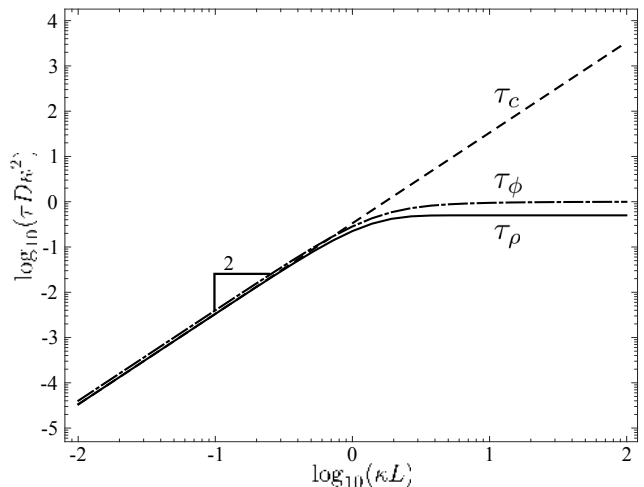
FIG. 2: Dimensionless time scales for charge density, \tau_\rho (solid), and salt concentration, \tau_c (dashed), at the cold electrode (the hot electrode exhibits identical timescales) as well as voltage, \tau_\phi (dot-dashed), versus \kappa L . For \kappa L \ll 1 , all time scales increase with a slope of 2. However, for \kappa L \gg 1 , the charge density and voltage time scales reach a constant value of 1/2 and 1 , respectively, but the concentration time scale continues to increase at the same rate.
