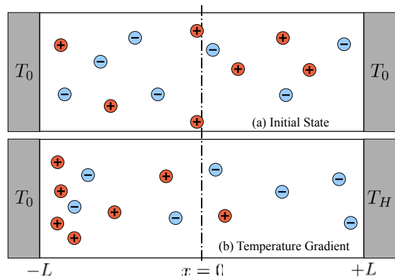
FIG. 1: Sketch of the model problem. The initial, isothermal state is depicted in figure (a); the charges are uniformly distributed. Upon heating the electrode at x = +L to a temperature T_H > T_0 , the charges migrate towards the colder regions of the cell, shown in figure (b). Two effects are depicted in (b): the concentration gradient and the regions of net charge near the electrodes.
