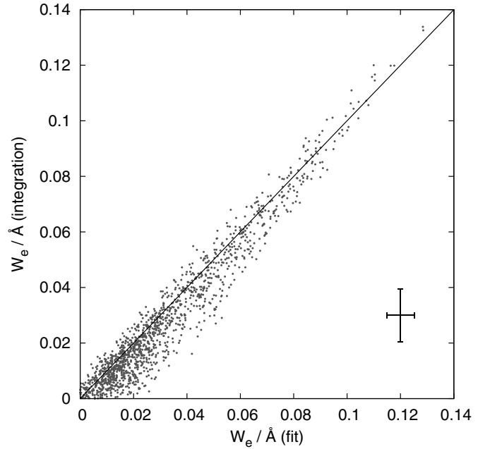
Figure 3. Correlation between fitted equivalent width and integrated equivalent width. The 1:1 correspondence is marked with a line. The typical error for each data point is marked with a cross. Data points are the same as used for Figures 8 and 9.
