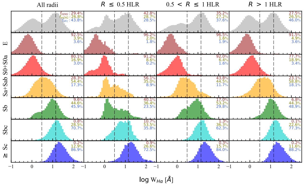
Figure 2. Distribution of W_{H\alpha} among 307958 zones of 391 CALIFA galaxies. Different rows show the breakdown of this distribution by Hubble type, from ellipticals (second row) to Sc and later (bottom). Results for the whole sample are shown in the top row. Histograms in the left-hand panels count all zones, while the others select different ranges in radius: the inner 0.5 HLR (second column), R = 0.5 –1 HLR (third), and outwards of 1 HLR (fourth). Vertical dashed lines mark the hDIG/mDIG and mDIG/SF frontiers at 3 and 14 Å, respectively. Labels on the top right of each panel list the fraction of the H\alpha flux associated with the hDIG, mDIG, and SF components (averaged over galaxies in each panel).
