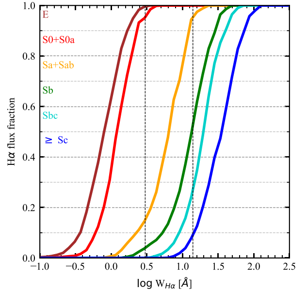
Figure 4. Cumulative fraction of the total galaxy H\alpha flux coming from regions with W_{H\alpha} smaller than a given value. The plot shows the median curves obtained for galaxies in six Hubble types.
