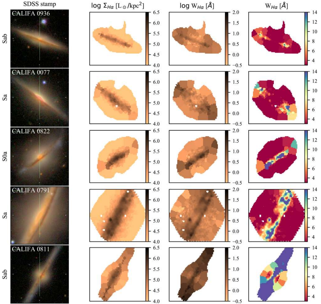
Figure 5. As Fig. 1, but for edge-on galaxies.
