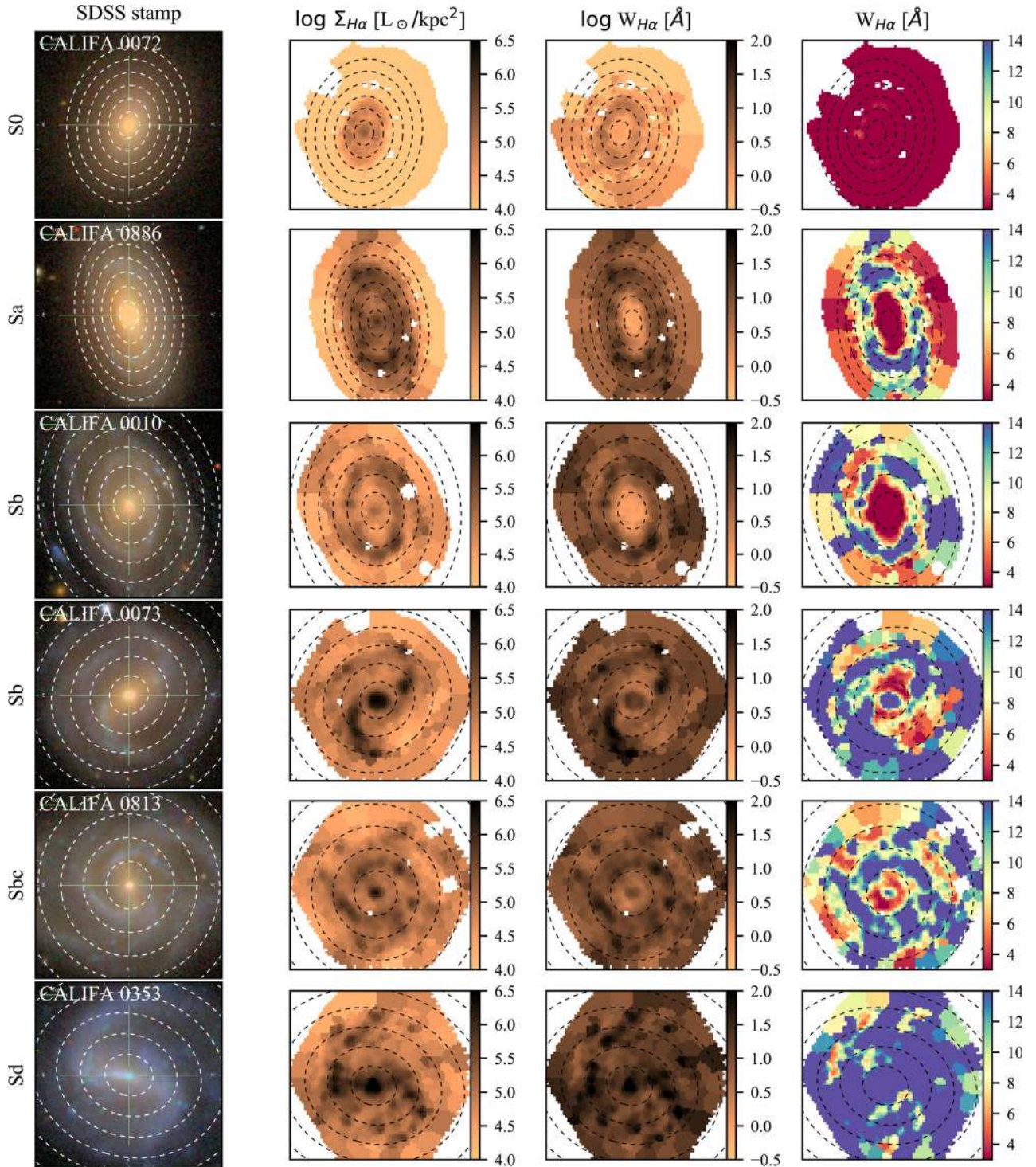
Figure 1. SDSS stamps, \Sigma_{H\alpha} , and W_{H\alpha} maps for example galaxies in CALIFA. Images on the right show W_{H\alpha} maps saturated at 3 and 14 Å, highlighting the proposed classification of hDIG, mDIG, and SFc. Dashed elliptical rings mark radial distances to the nucleus of R = 0.5, 1.0, 1.5, \dots in units of the galaxy's half-light radius (HLR). Empty patches mask foreground sources and other artefacts.
