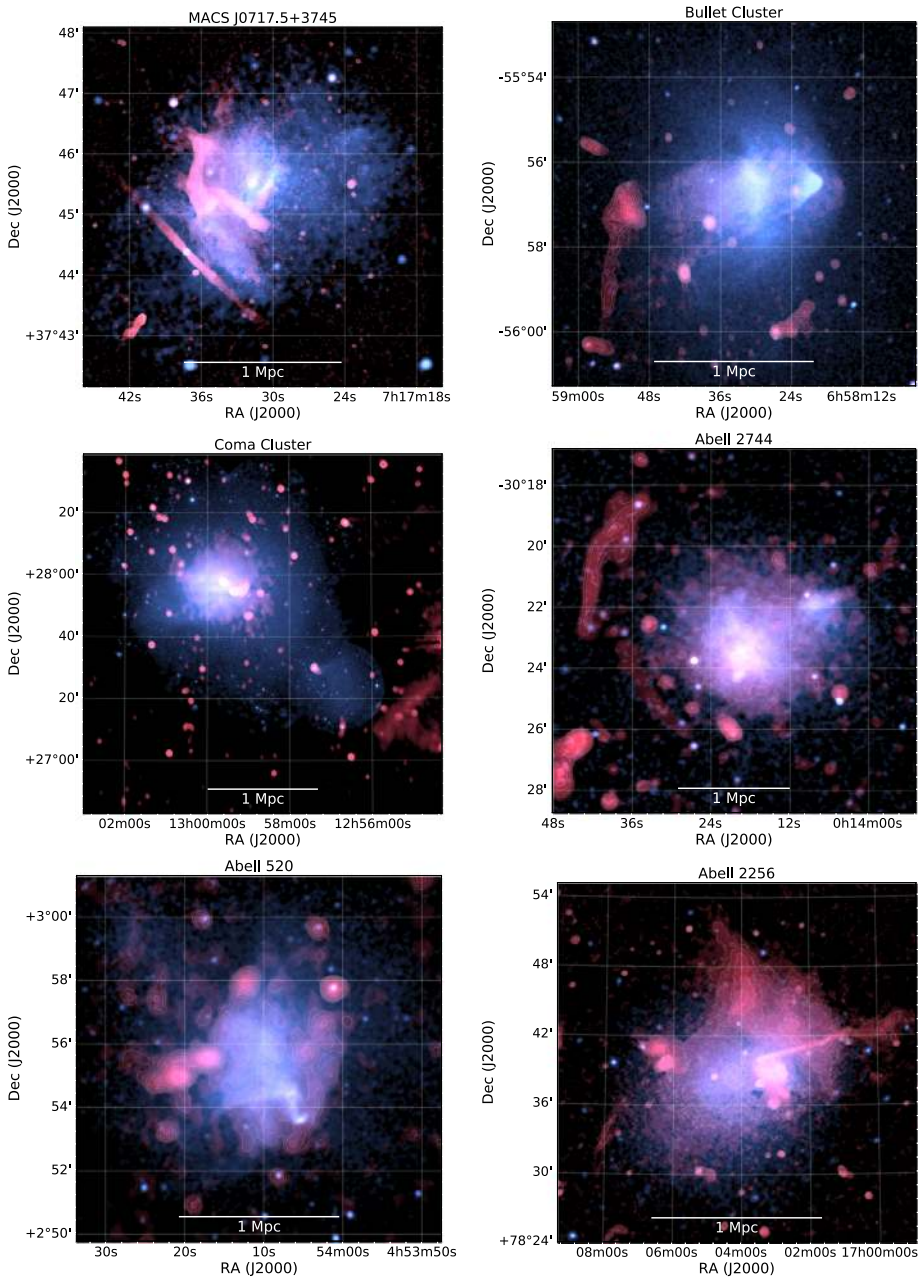
Fig. 6 Examples of clusters hosting giant radio halos. The radio emission is shown in red and the X-ray emission in blue. MACS J0717.5+3745: VLA 1–6 GHz and Chandra 0.5–2.0 keV (van Weeren et al. 2017a). Bullet cluster: ATCA 1.1–3.1 GHz and Chandra 0.5–2.0 keV (Shimwell et al. 2015; Andrade-Santos et al. 2017). Coma cluster: WSRT 352 MHz and XMM-Newton 0.4–1.3 keV (Brown and Rudnick 2011). Abell 2744: VLA 1–4 GHz and Chandra 0.5–2.0 keV (Pearce et al. 2017). Abell 520: VLA 1.4 GHz and Chandra 0.5–2.0 keV (Wang et al. 2018; Andrade-Santos et al. 2017). Abell 2256: LOFAR 120–170 MHz and XMM-Newton 0.4–1.3 keV (van Weeren et al. in prep)
