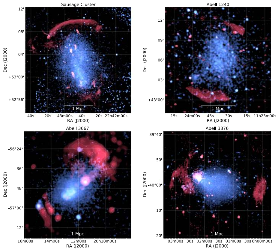
Fig. 18 Examples of cluster double radio shocks. The radio emission is shown in red and the X-ray emission in blue. Sausage Cluster: GMRT 610 MHz and Chandra 0.5–2.0 keV (van Weeren et al. 2010; Ogrea et al. 2014a). Abell 1240: LOFAR 120–168 MHz and Chandra 0.5–2.0 keV (Hoang et al. 2018b). Abell 3667: MWA 170–231 MHz and ROSAT PSPC (Hurley-Walker et al. 2017; Voges et al. 1999). Abell 3376: GMRT 317 MHz and XMM-Newton 0.3–2.0 keV (Kale et al. 2012; Urdampilleta et al. 2018)
