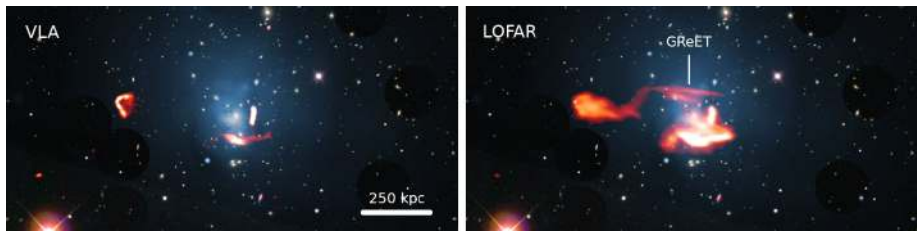
Fig. 31 Optical image of the galaxy cluster Abell 1033, with over plotted in blue the X-ray emission and in orange the synchrotron radio emission. The left panel shows our view of the galaxy cluster at conventional radio frequencies (VLA at 1.4 GHz). The right panel shows the discovery of the first GRrET (gently re-energized radio tail), a new type of radio source visible uniquely at very low frequencies (LOFAR at 140 MHz; de Gasperin et al. 2017a). To detect the GRrET at 1.4 GHz would require a century of VLA observing time
