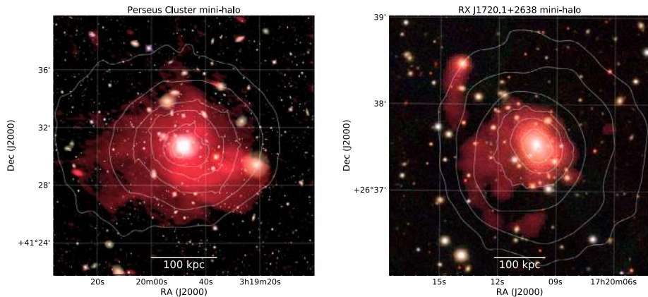
Fig. 12 Radio-optical overlays of the mini-halos in the Perseus cluster ( left ) and RX J1720.1+2638 ( right ). Both mini-halos display clear substructure. X-ray surface brightness contours are shown in white. The X-ray and radio data are the same as listed in Fig. 11. The optical images are taken from SDSS (Perseus; gri bands, Abolfathi et al. 2018) and Pan-STARRS (RX J1720.1+2638; grz bands, Chambers et al. 2016)
