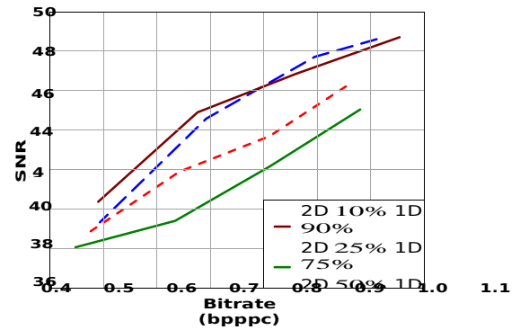
Fig. 3: Different distributions of the known data for AVIRIS Yellowstone sc 00 Radiance (224 components).
