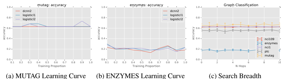
Figure 3: Learning curves for the MUTAG (3a) and ENZYMES (3b) datasets as well as the effect of search breadth (3c)
