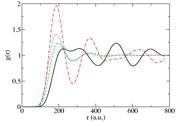
FIG. 9. Parallel and antiparallel spin PCF's in the antiferromagnetic crystal and unpolarized fluid at r_s = 110 . Solid line: parallel spin crystal PCF; dashed line: parallel spin fluid PCF; dash-dotted line: antiparallel spin crystal PCF; dotted line: antiparallel spin fluid PCF. The statistical errors are less than 0.005.
