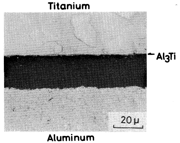
Photo. 3 Cross sectional microstructure of the fractured zone obtained from the joint which had much lower tensile strength than the base metals. The welding temperature, time, and pressure were 600°C, 10 min, and 0 kg/mm 2 , respectively.
