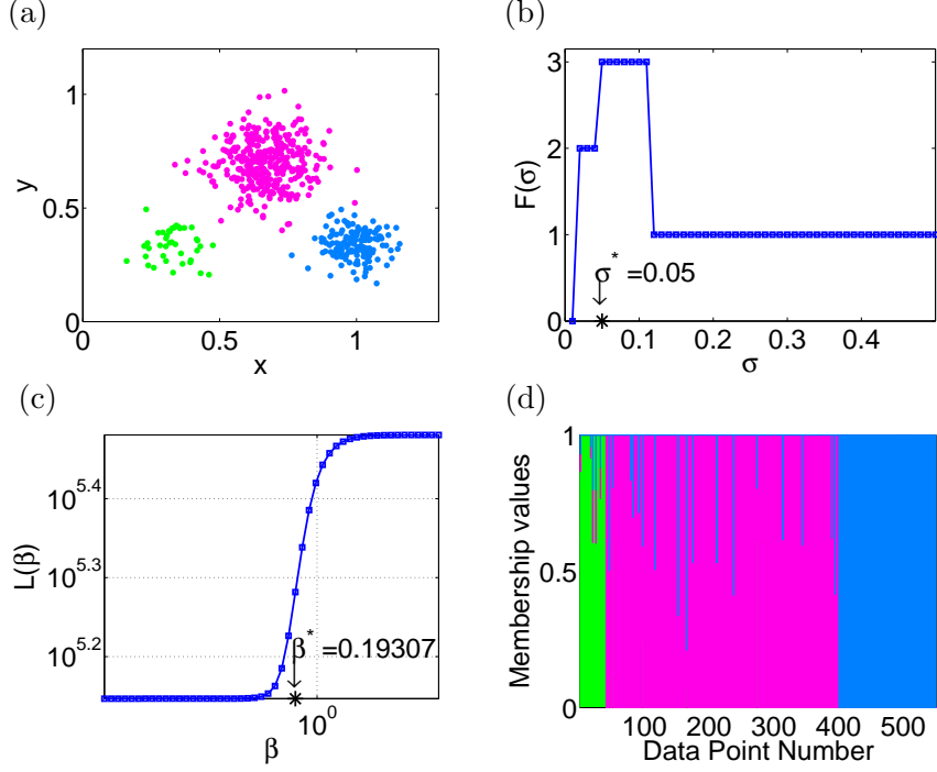
Figure 1: (a) “Globular clusters” data set. (b) F(\sigma) for the data set in (a). For this data set we determined the number of clusters C to be 3, and \sigma^* = 0.05 , for the parameter M = 35 . (c) L(\beta) , given by Eq. (4) plotted on a logarithmic scale, for the data set in (a). \beta^* = 0.19307 was obtained using Eq. (5). (d) DifFUZZY membership values for this data set. Each data point is represented by a bar of total height equal to 1 (from Eq. 2). ( M = 35 ). Colour code: green, red and blue correspond to the membership value of the data points in the three clusters, with the corresponding colour code as in (a). This representation will be used in Figs. 2 and 3.
