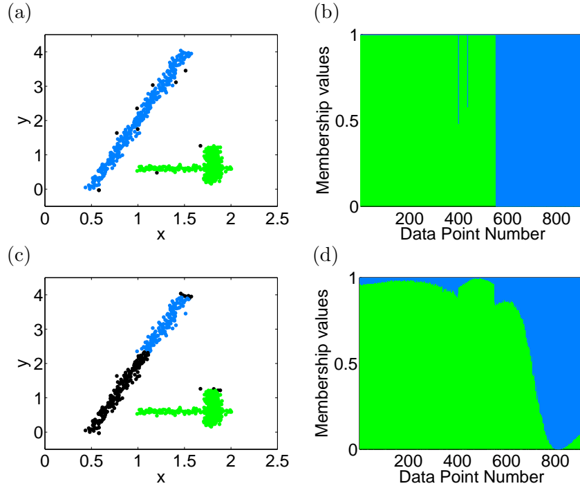
Figure 3: “Elongated clusters” test data set. (a) DifFUZZY HCT-plot , z = 0.9 . ( M = 150 ). (b) DifFUZZY membership values . ( M = 150 ). (c) FCM HCT-plot , z = 0.9 . (d) FCM membership values . Colour code for (b) and (d) as in Fig. 1(b).
