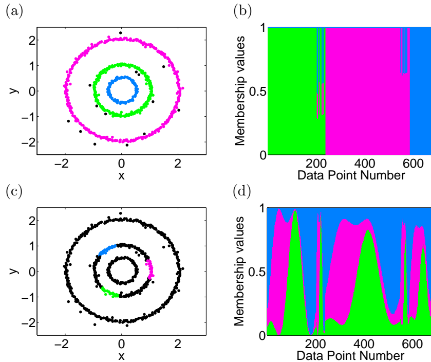
Figure 2: “Concentric rings” test data set. (a) DiffFUZZY HCT-plot, z = 0.9 . ( M = 90 ). (b) DiffFUZZY membership values. (c) FCM HCT-plot, z = 0.9 . (d) FCM membership values. Colour code for (b) and (d) as in Fig. 1(b).
