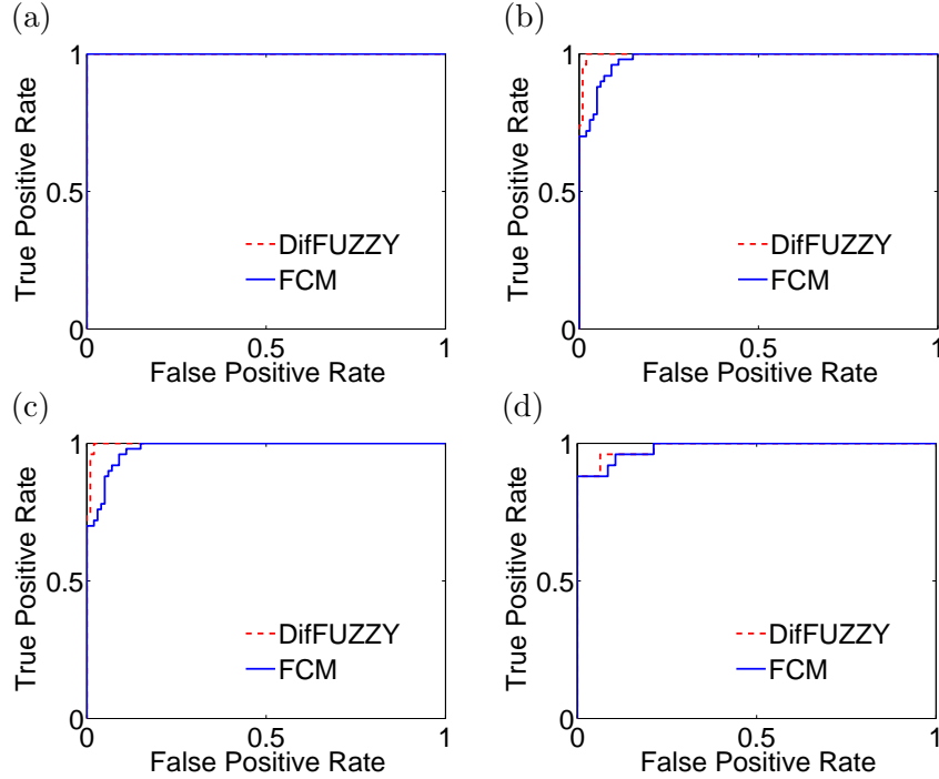
Figure 4: DifFUZZY and FCM ROC curves for (a) the Iris Setosa data ( M = 15 ), (b) the Iris Versicolor data ( M = 15 ), (c) the Iris Virginica data ( M = 15 ) and (d) the Leukemia data set ( M = 11 ).
