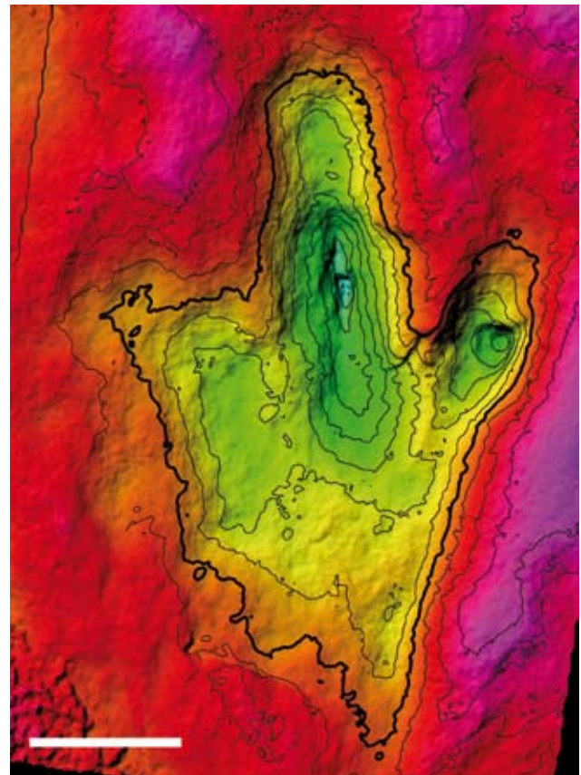
Fig. 14 - Superimposition of the contour map by laser scanner and photogrammetry derived 3D model. Scale bar 5 cm.
