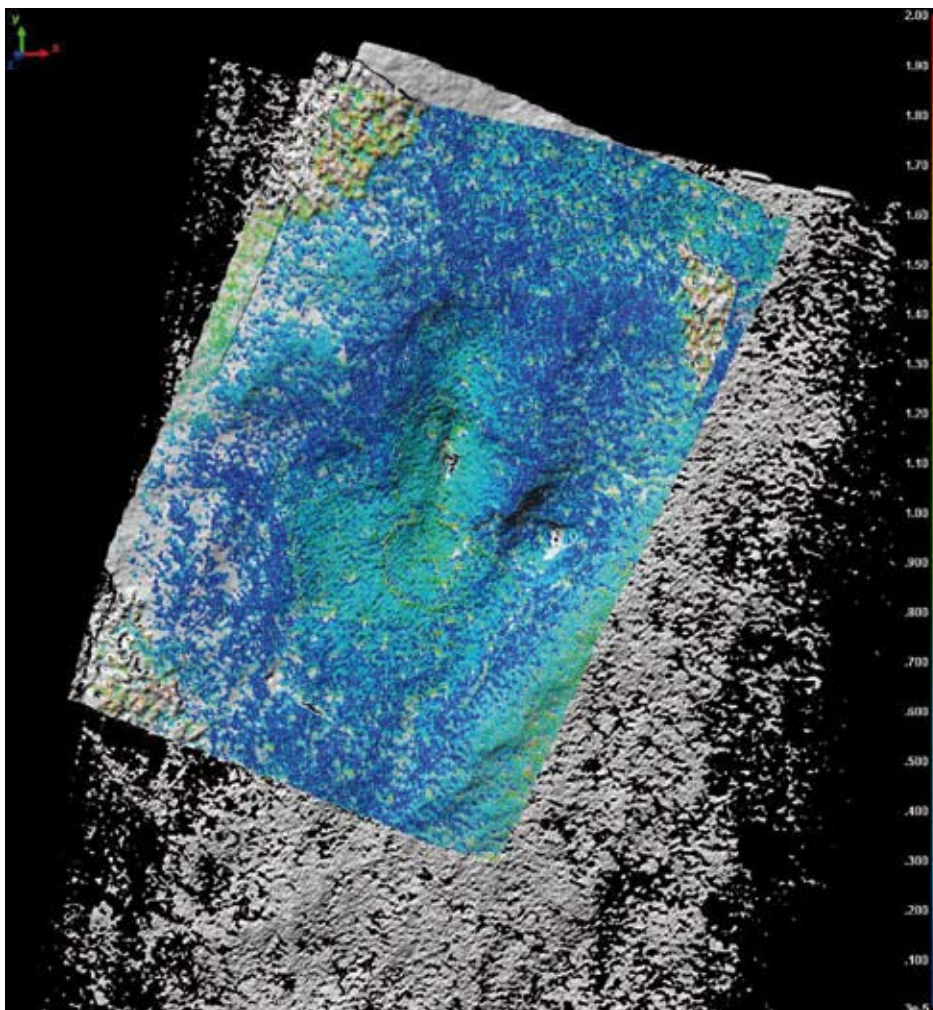
Fig. 15 - Colour-coded difference between the laser scanner and photogrammetric models. Note as in the track area the difference between the two models is on average less than 1 mm.
