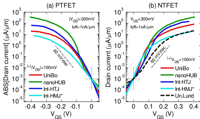
Figure 5: (a) p -type and (b) n -type transfer-characteristics ( I_D - V_{GS} ) at |V_{DS}| = 300 mV of virtual p/n -TFETs presented in [59] (UniBo, devices used in this work), of the template used in [68] (nanoHUB), the templates in [14] (Intel-HTJ), [ ] (Intel-HMJ), at |V_{DS}| = 100 mV) and of the experimental n -TFET in [7] (Un.Lund). For a fair comparison, the I_D - V_{GS} characteristics have been normalized by the gate perimeter and aligned at the same I_{off} = 1nA/\mu m .
