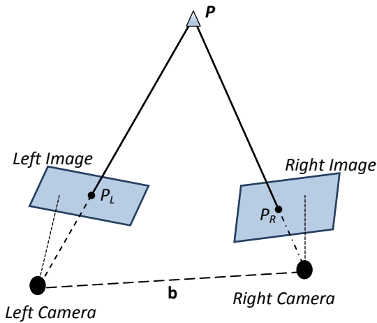
Figure 1. Epipolar geometry
