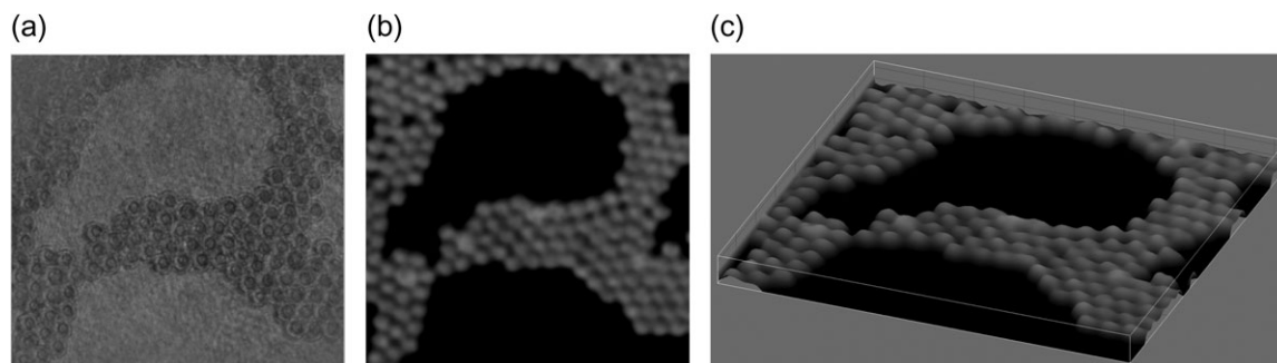
Fig. 3. (a) Intensity and (b) phase images of polystyrene beads whose diameters are 5 \mu\text{m} , which are obtained with a hologram at a wavelength of 532 nm. (c) 3D rendering image obtained from (b).
