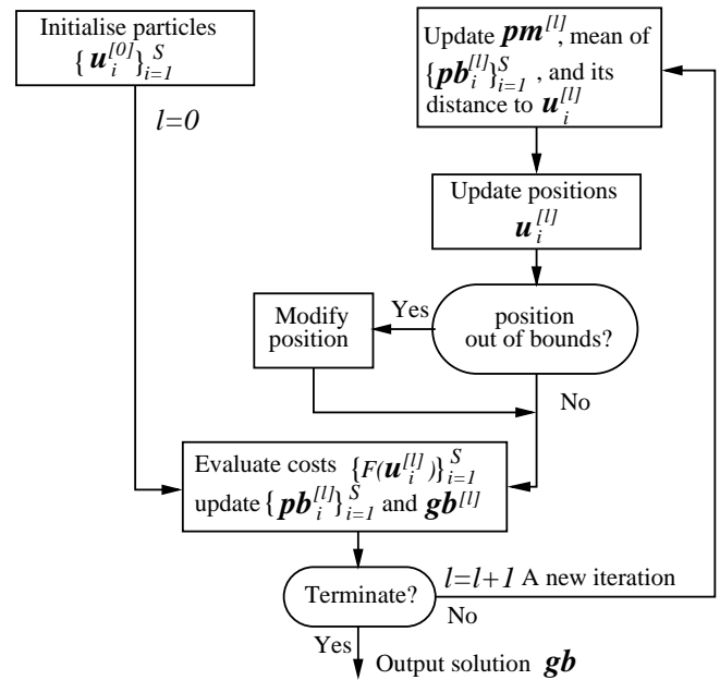
Figure 2 Flowchart of the QPSO algorithm
