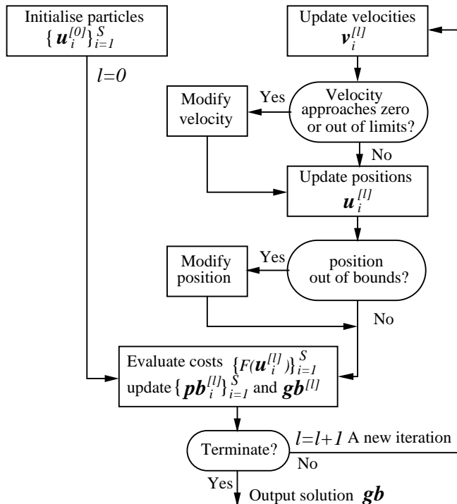
Figure 1 Flowchart of the PSO algorithm
